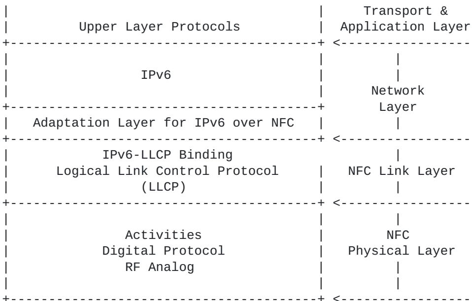
Figure 2: Protocol Stacks for IPV6 over NFC
