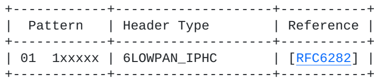
Figure 6: Dispatch Values
