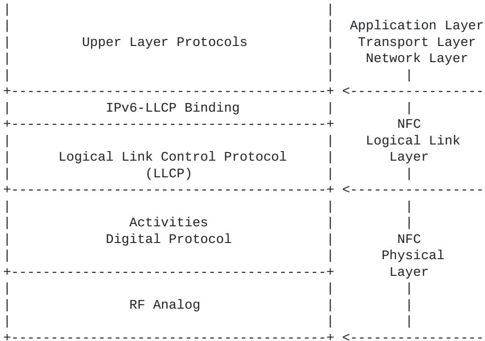
Figure 1: Protocol Stacks of NFC
