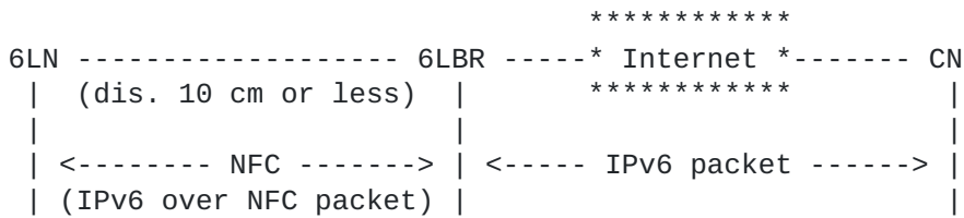
Figure 10: NFC-enabled device network connected to the Internet
