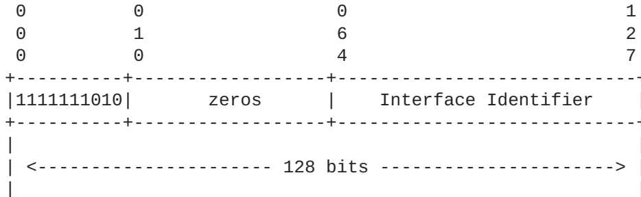
Figure 4: IPv6 link-local address in NFC
