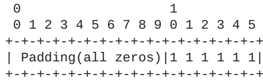
Figure 9: Multicast address mapping
