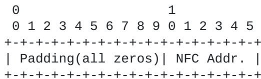
Figure 7: NFC short address format
