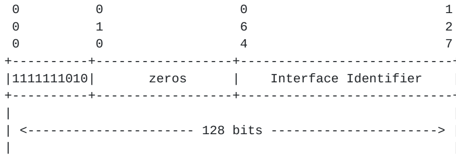
Figure 5: IPv6 link-local address in NFC
