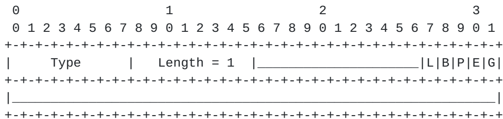
Figure 1: New capability Bits L, B, P, E in the CIO
