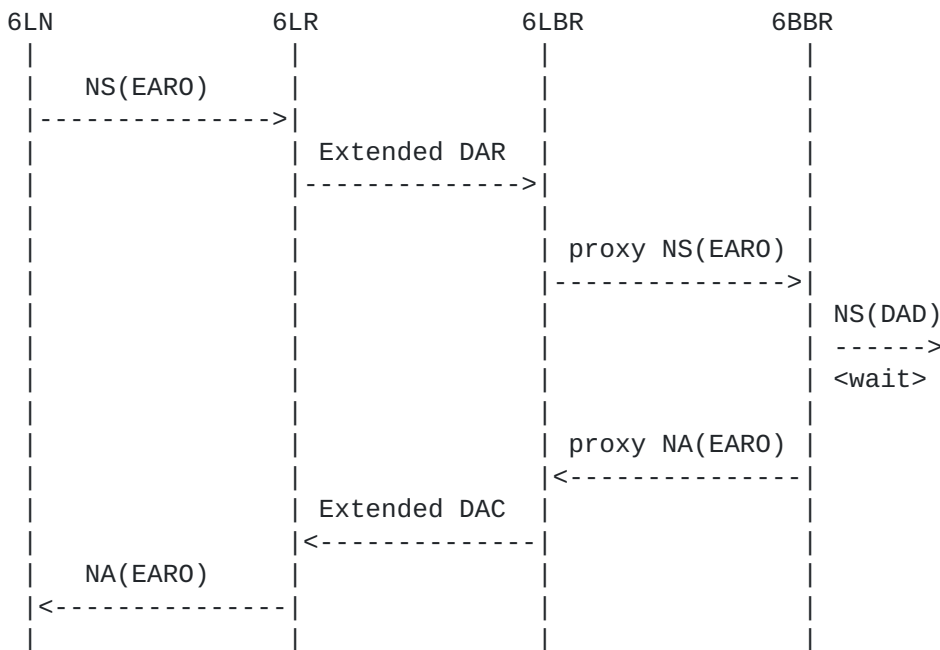
Figure 1: (Re-)Registration Flow
