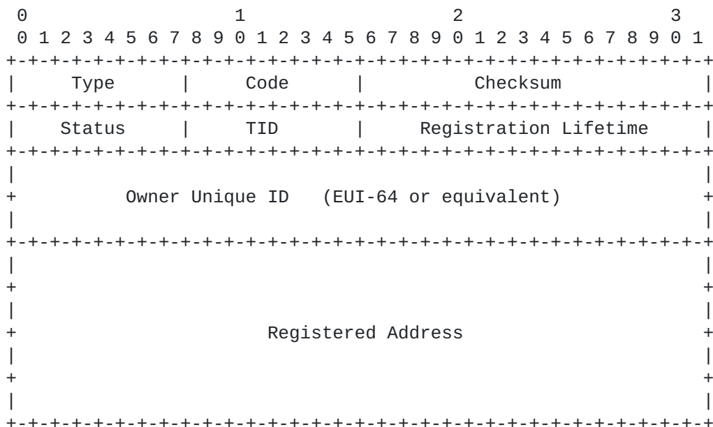
Figure 3: Duplicate Address Messages Format
