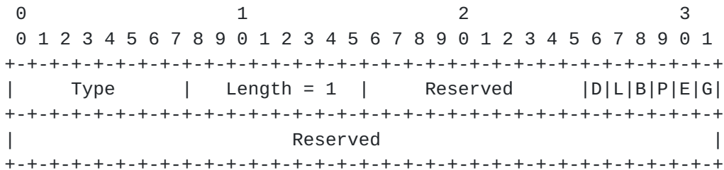
Figure 3: New capability Bits L, B, P, E in the 6CIO
