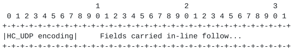
Figure 16: HC_UDP (UDP common compressed header encoding)
