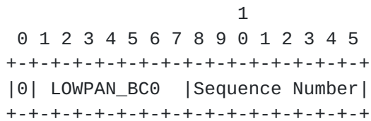
Figure 17: Broadcast Header
