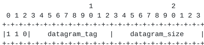
Figure 10: First Fragment
