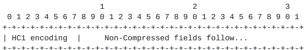
Figure 15: LOWPAN_HC1 (common compressed header encoding)
