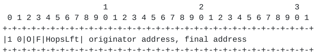
Figure 9: Mesh Addressing Type and Header
