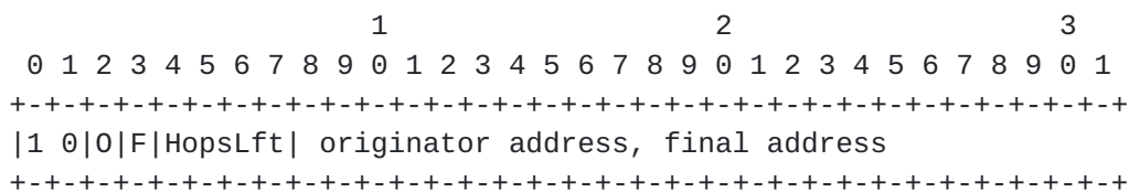
Figure 9: Mesh Addressing Type and Header
