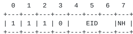
Figure 6: IPv6 Extension Header Encoding
