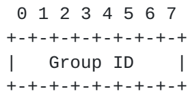
Figure 9: DAM = 11. 8-bit Compressed Multicast Address (FF02::gg).
