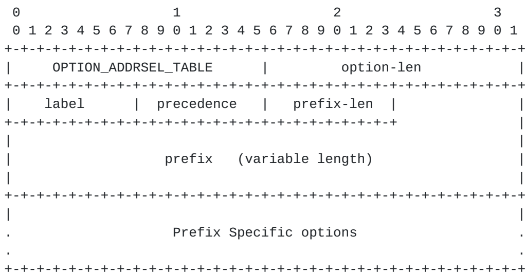
Figure 2: Address Selection Policy Table option format
