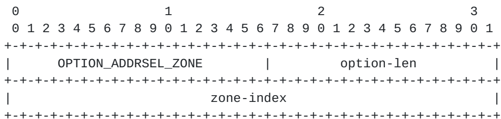
Figure 3: Zone Index option format
