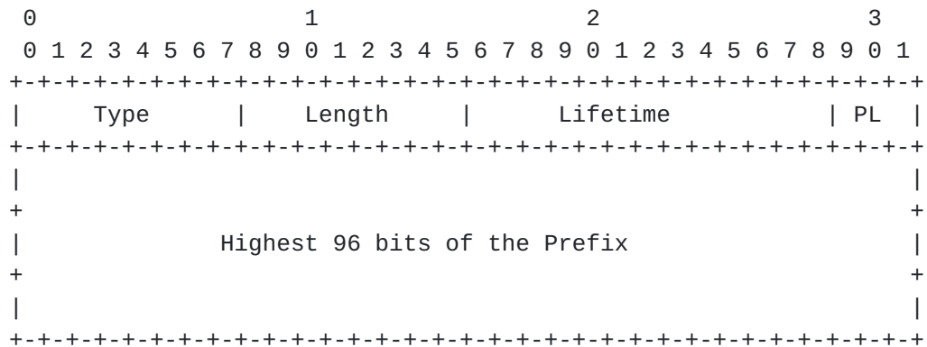
Figure 1: NAT64 Prefix Option Format
