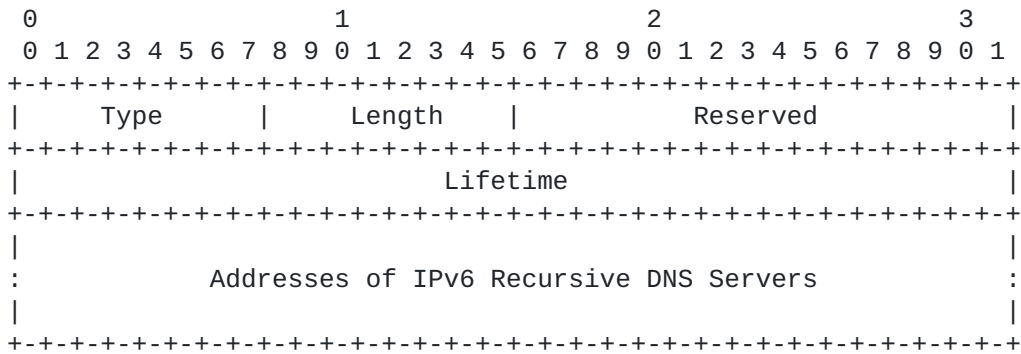
Figure 1: Recursive DNS Server (RDNSS) Option Format
