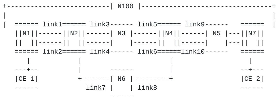
Figure 1 Reference Topology
