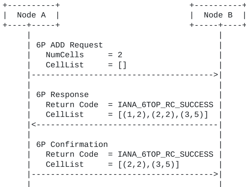
Figure 5: A 3-step 6P transaction.
