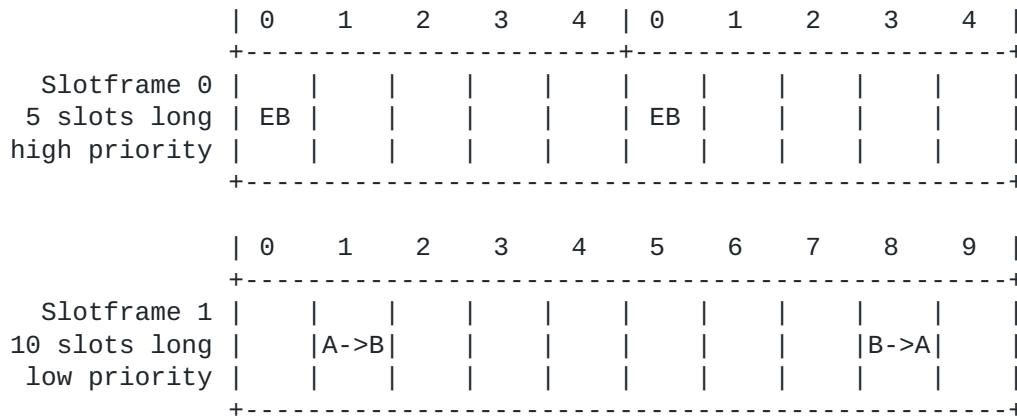
Figure 3: 2-slotframe structure when using 6top alongside the Minimal 6TiSCH Configuration.
