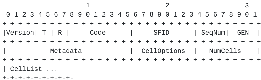
Figure 9: 6P ADD Request Format.
