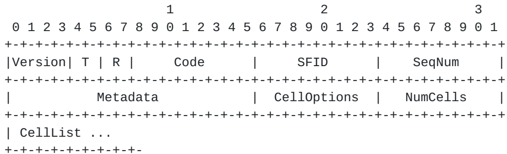
Figure 11: 6P DELETE Request Format.
