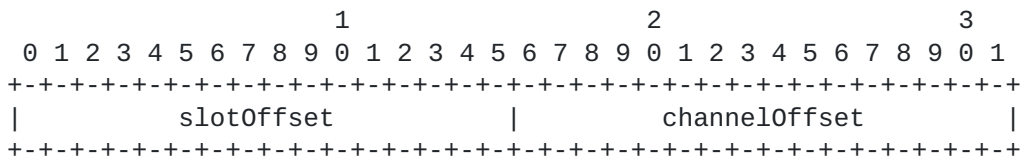
Figure 8: 6P Cell Format.
