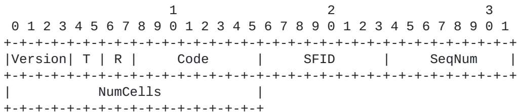
Figure 20: 6P COUNT Response Format.
