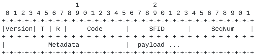
Figure 25: 6P SIGNAL Request Format.
