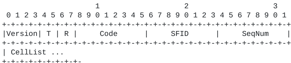
Figure 14: 6P RELOCATE Response and Confirmation Formats.
