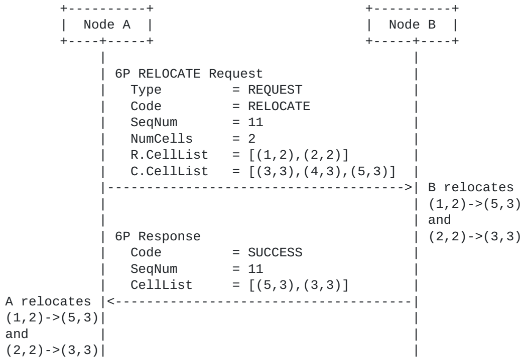
Figure 15: Example of a successful 2-step 6P RELOCATION Transaction.
