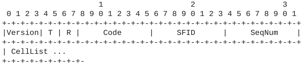
Figure 22: 6P LIST Response Format.
