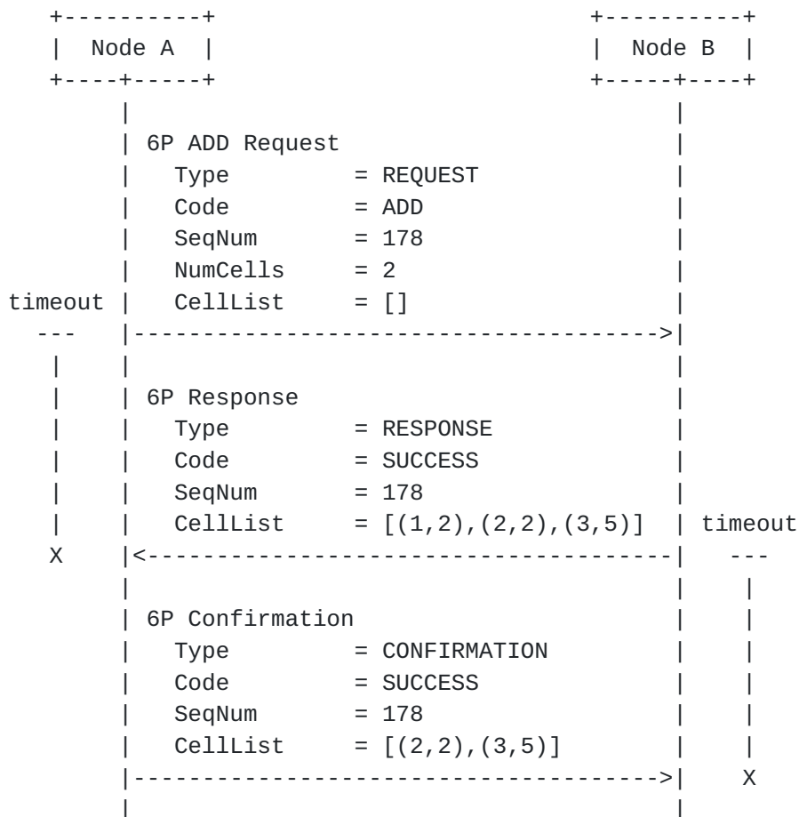
Figure 5: An example 3-step 6P Transaction.
