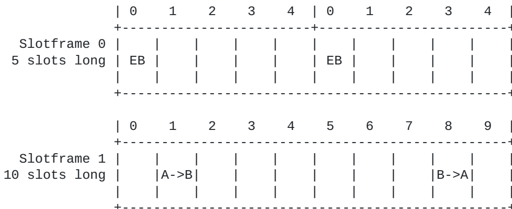
Figure 3: 2-slotframe structure when using 6P alongside the Minimal 6TiSCH Configuration.
