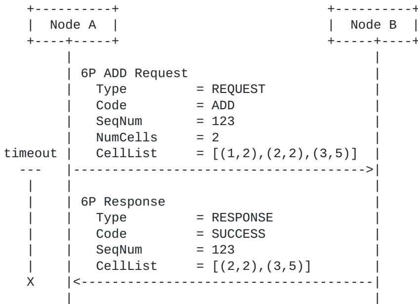
Figure 4: An example 2-step 6P Transaction.
