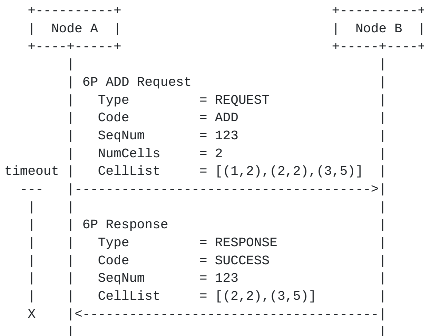
Figure 4: An example 2-step 6P Transaction.
