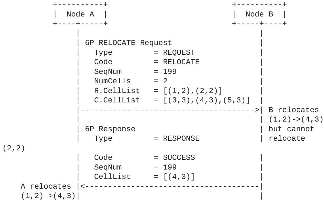
Figure 16: Example of a partially successful 2-step 6P RELOCATION Transaction.
