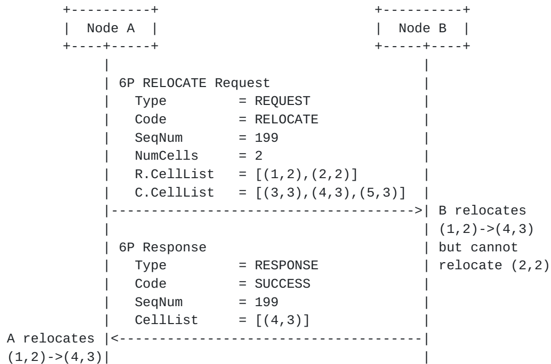
Figure 16: Example of a partially successful 2-step 6P RELOCATION Transaction.
