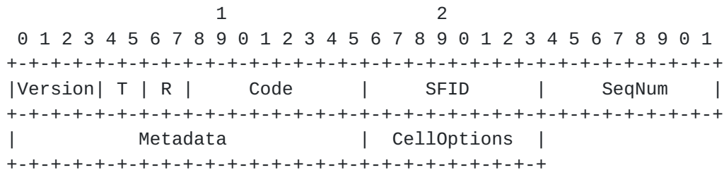
Figure 19: 6P COUNT Request Format.
