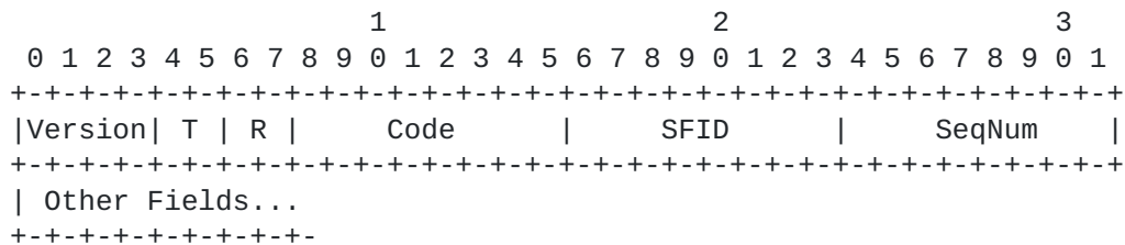
Figure 6: Generic 6P Message Format.
