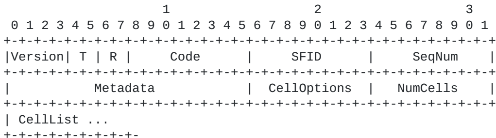
Figure 9: 6P ADD Request Format.
