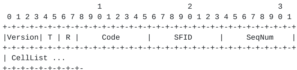
Figure 12: 6P DELETE Response and Confirmation Formats.
