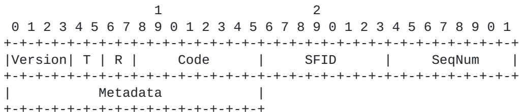
Figure 23: 6P CLEAR Request Format.
