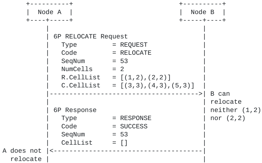
Figure 17: Failed 2-step 6P RELOCATION Transaction Example.
