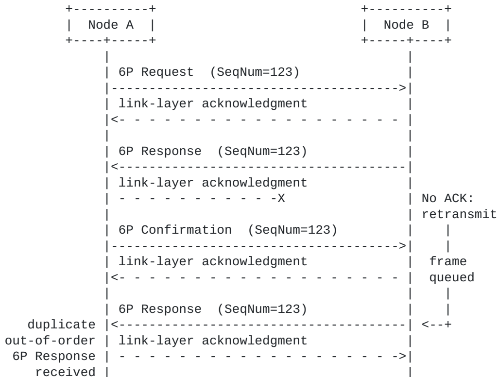
Figure 29: Example out-of-order duplicate 6P message.
