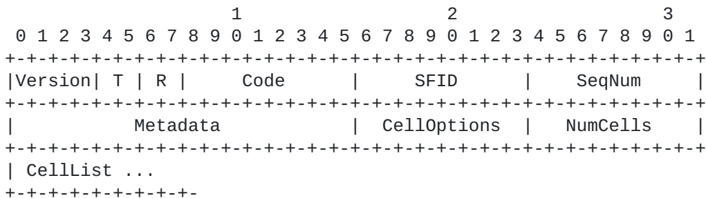
Figure 11: 6P DELETE Request Format.
