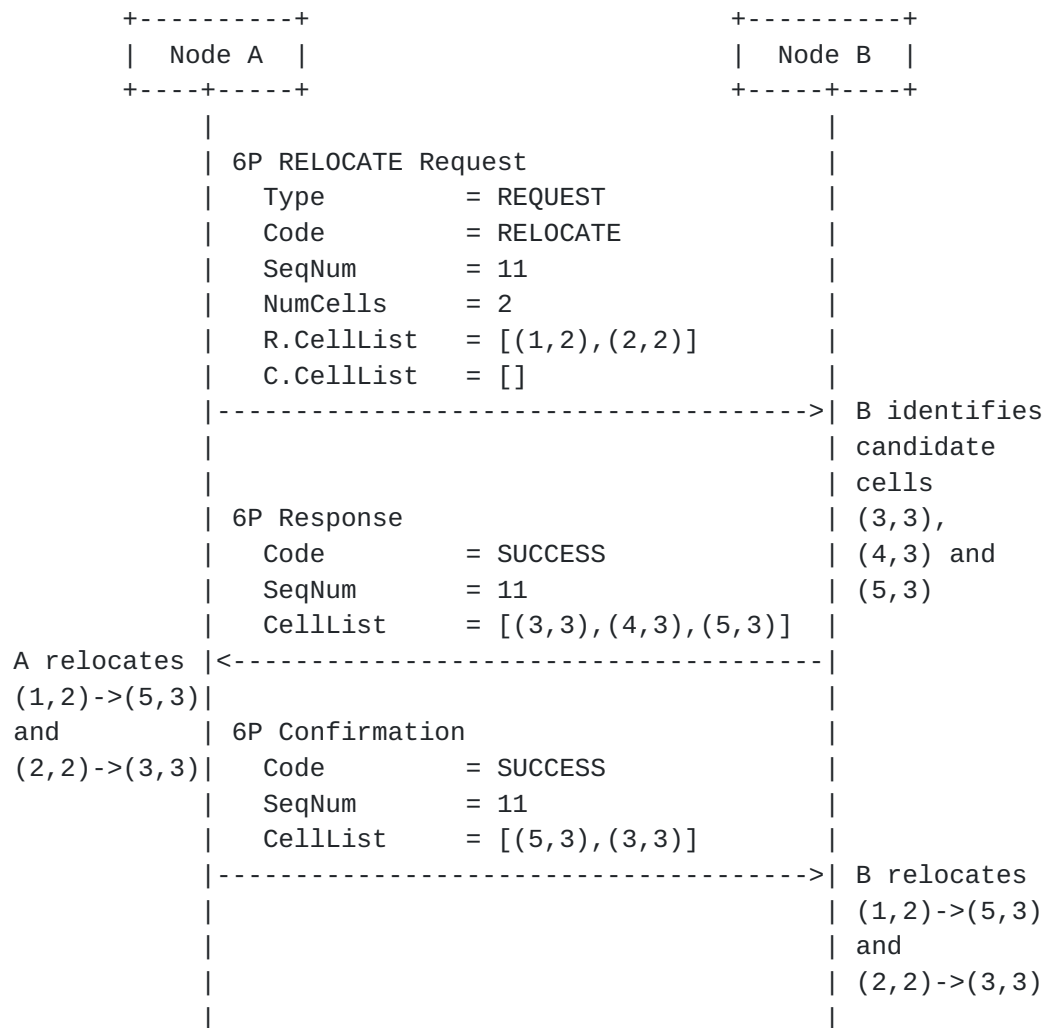
Figure 18: Example of a successful 3-step 6P RELOCATION Transaction.
