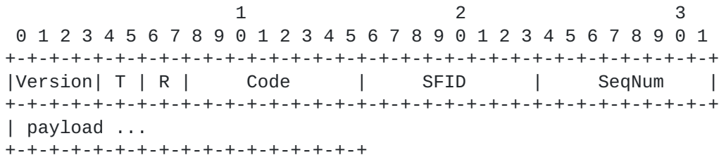
Figure 26: 6P SIGNAL Response Format.
