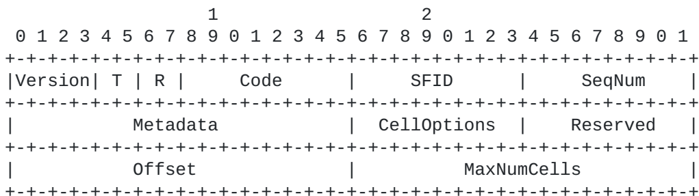
Figure 21: 6P LIST Request Format.
