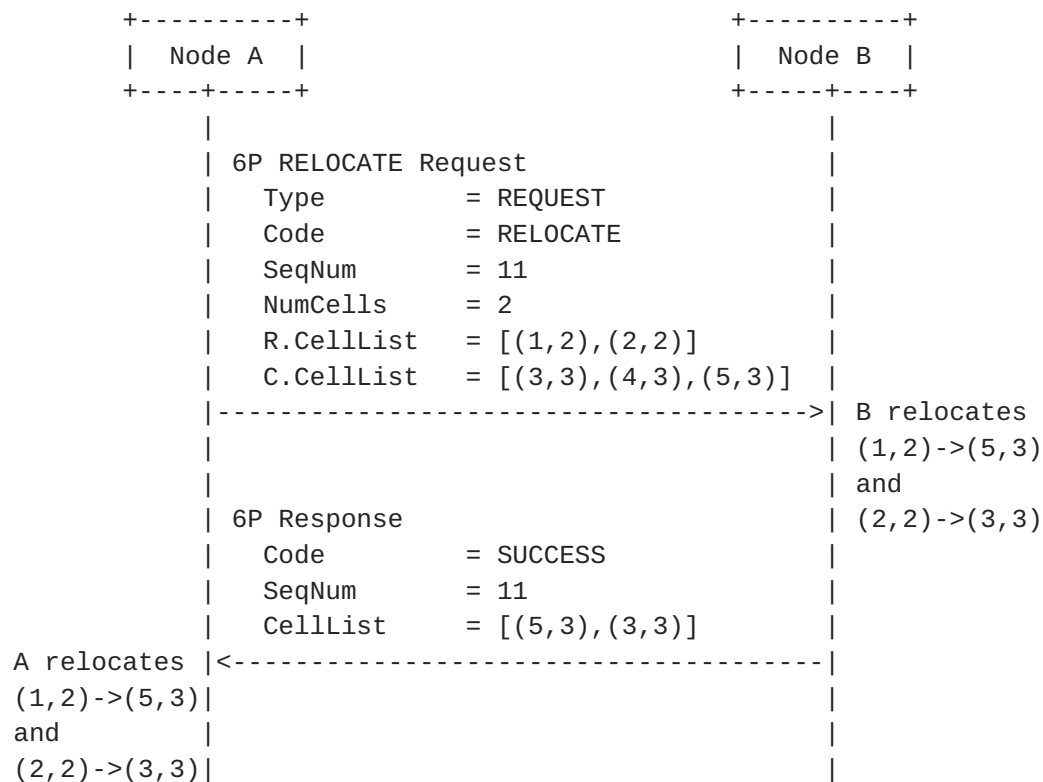
Figure 15: Example of a successful 2-step 6P RELOCATION Transaction.
