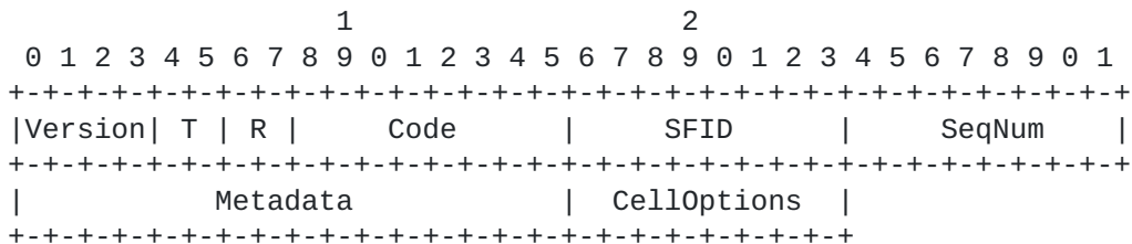
Figure 19: 6P COUNT Request Format.
