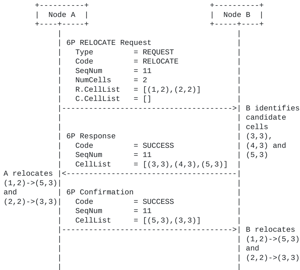
Figure 18: Example of a successful 3-step 6P RELOCATION Transaction.
