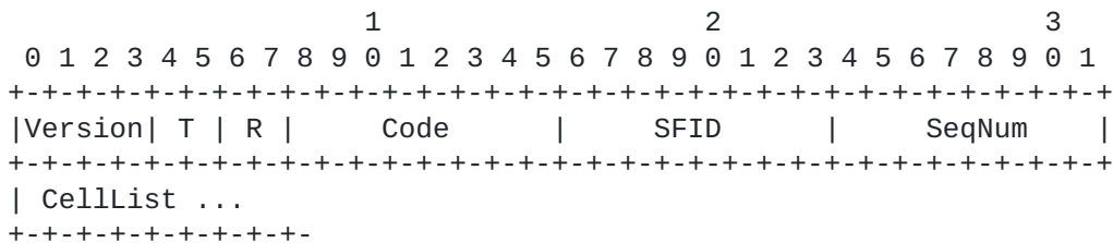
Figure 12: 6P DELETE Response and Confirmation Formats.
