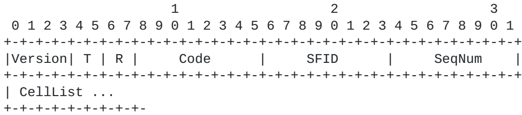
Figure 10: 6P ADD Response and Confirmation Formats.
