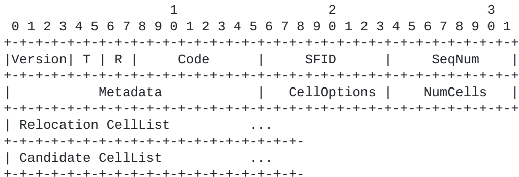
Figure 13: 6P RELOCATE Request Format.
