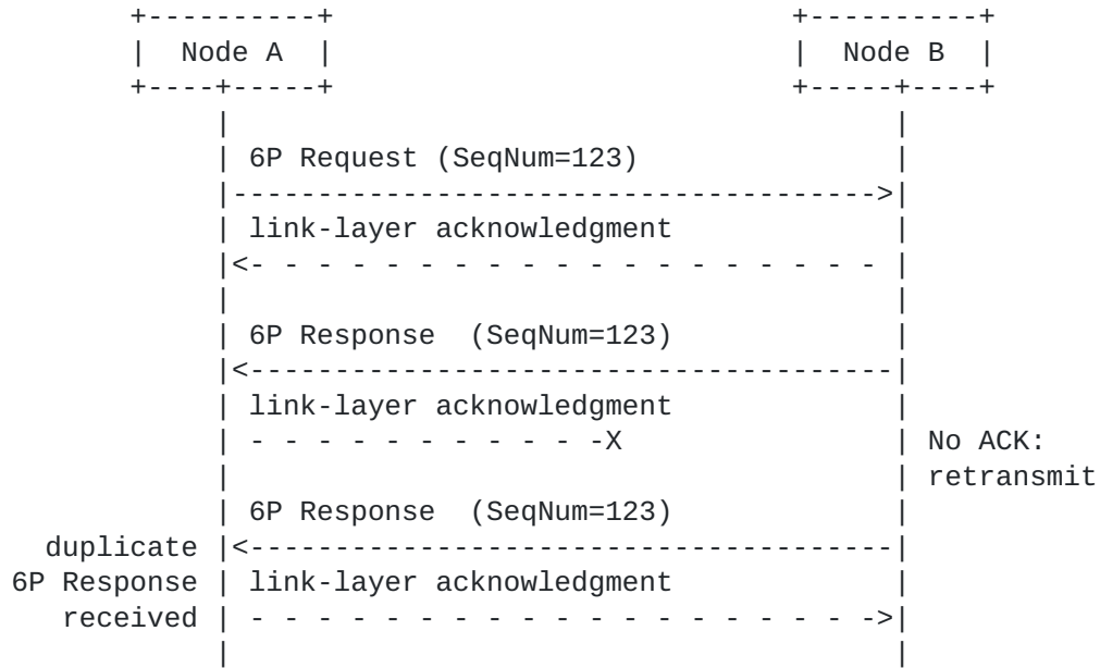
Figure 28: Example duplicate 6P message.
