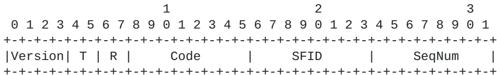
Figure 24: 6P CLEAR Response Format.
