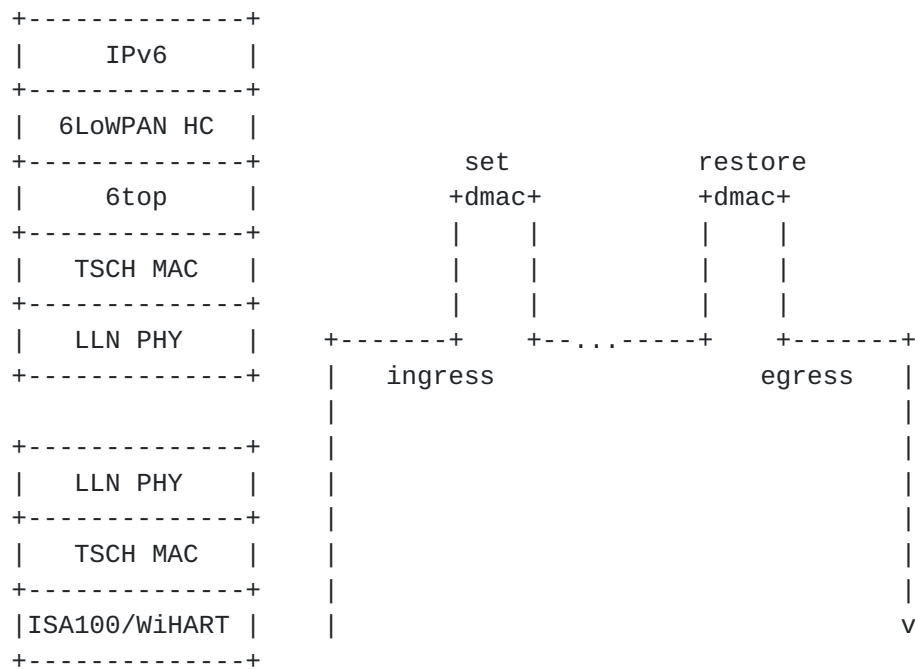
Figure 5: Track Forwarding, Tunnel Mode
