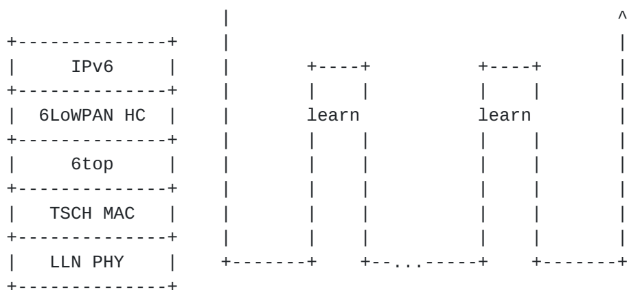
Figure 6: Forwarding First Fragment
