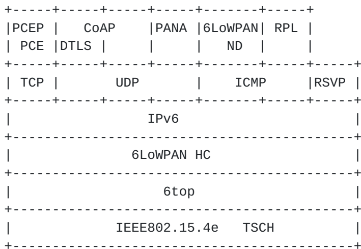
Figure 3: 6TiSCH stack
