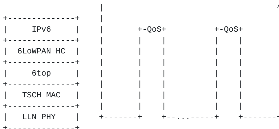
Figure 8: IP Forwarding
