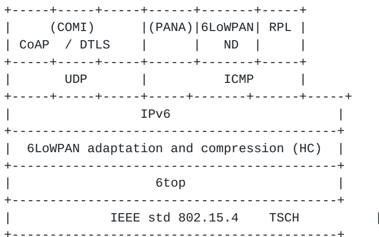
Figure 1: 6TiSCH Protocol Stack
