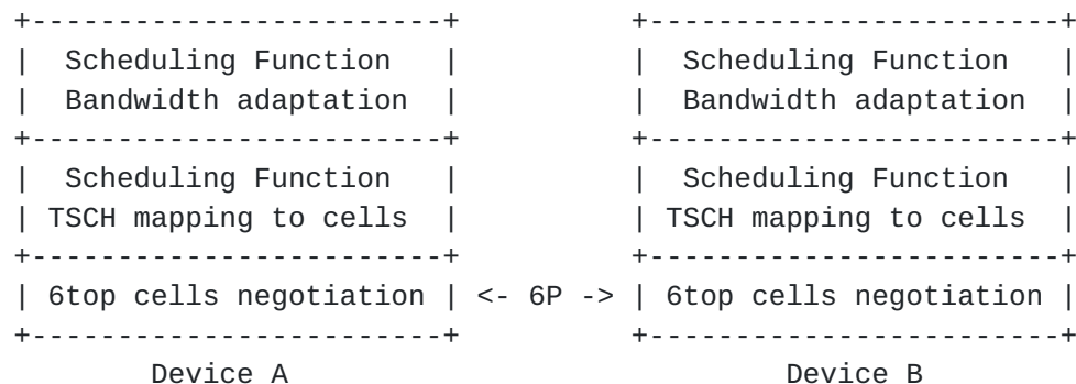
Figure 6: SF/6P stack in 6top
