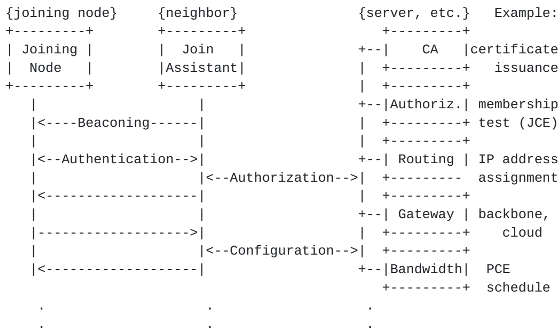
Figure 14: Network joining, with only authorization by third party
