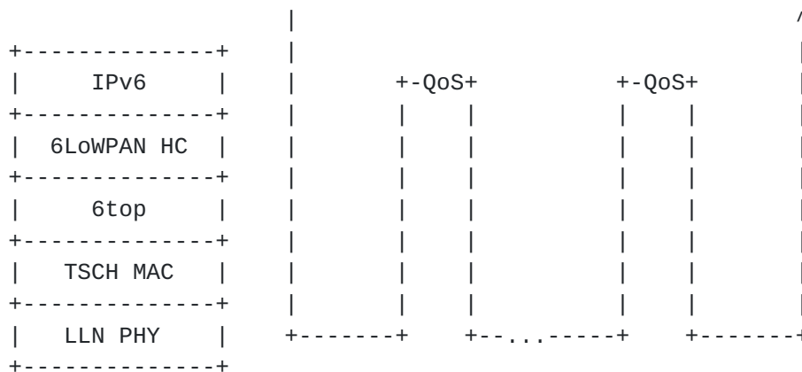
Figure 15: IP Forwarding
