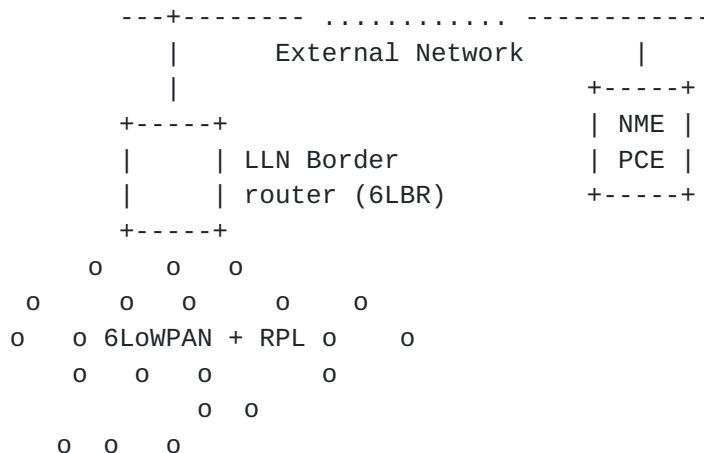
Figure 1: Basic Configuration of a 6TiSCH Network
