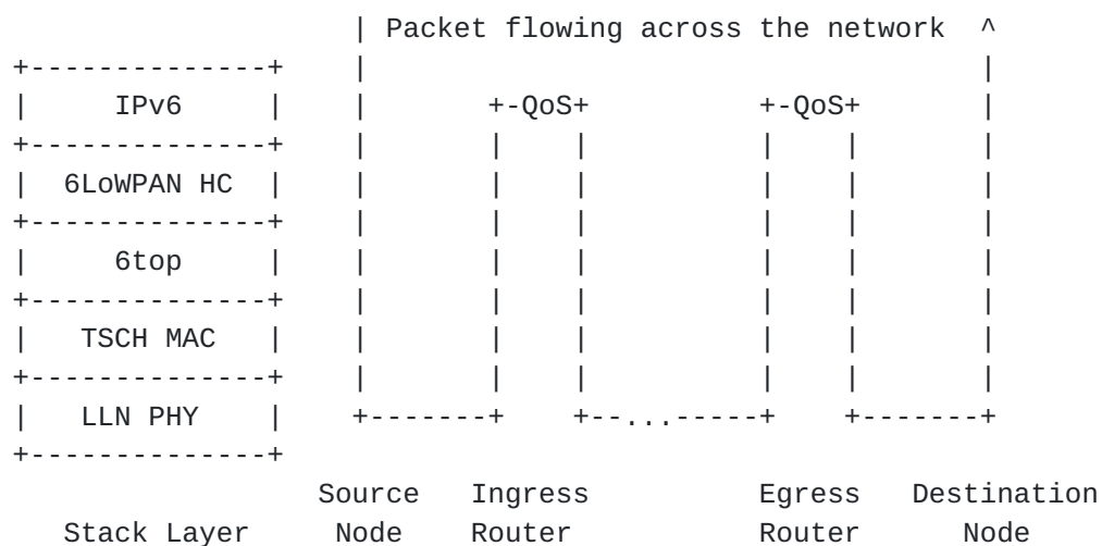
Figure 14: IP Forwarding
