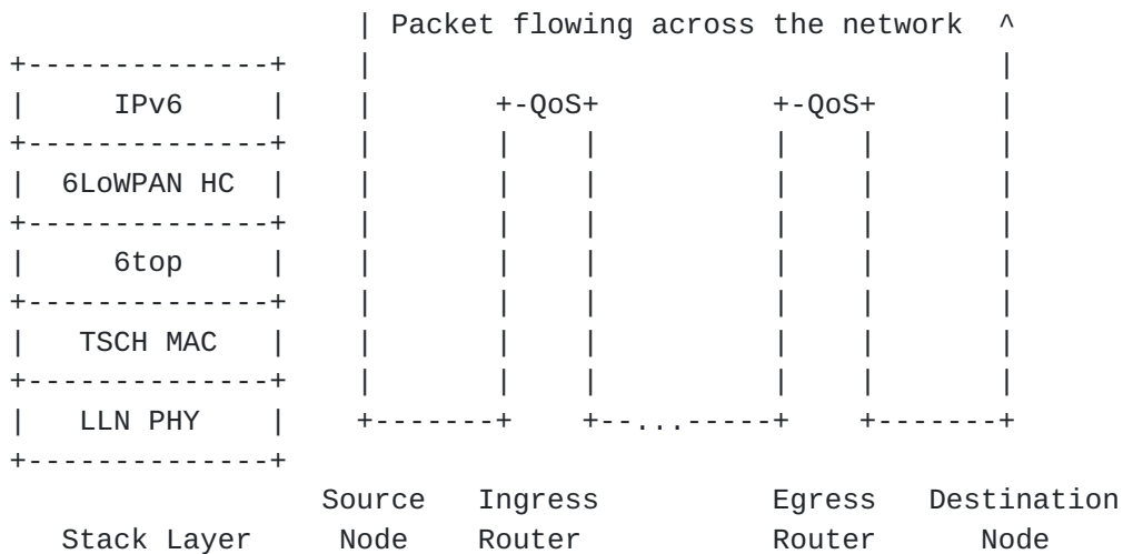
Figure 14: IP Forwarding
