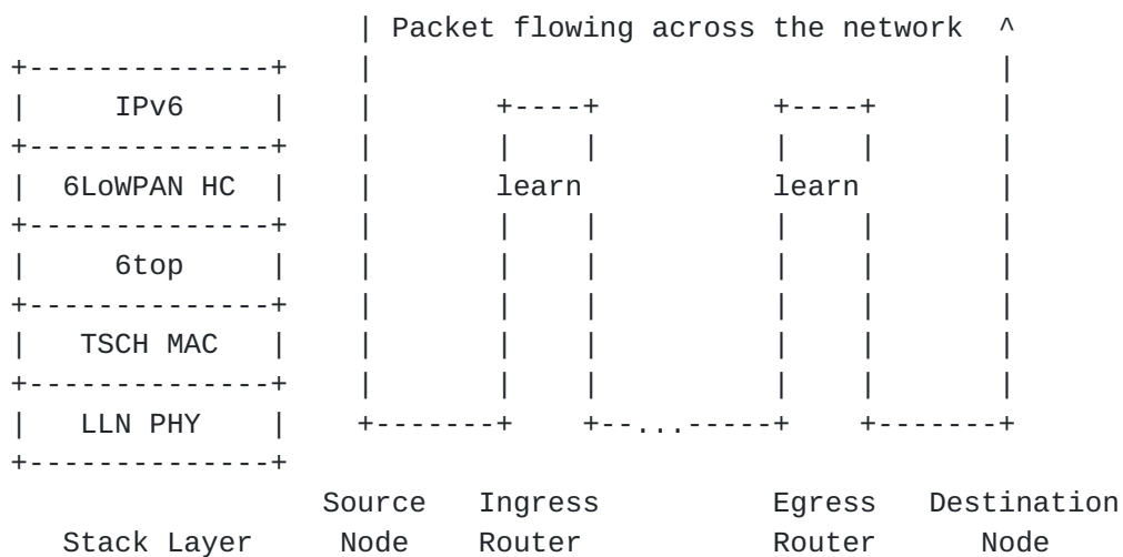
Figure 15: Forwarding First Fragment
