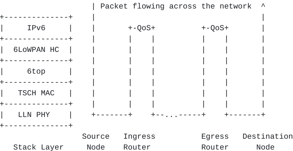
Figure 14: IP Forwarding
