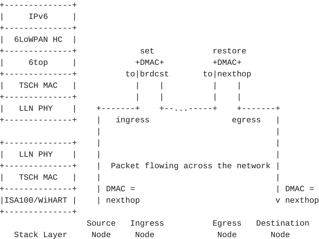
Figure 13: Track Forwarding, Tunnel Mode
