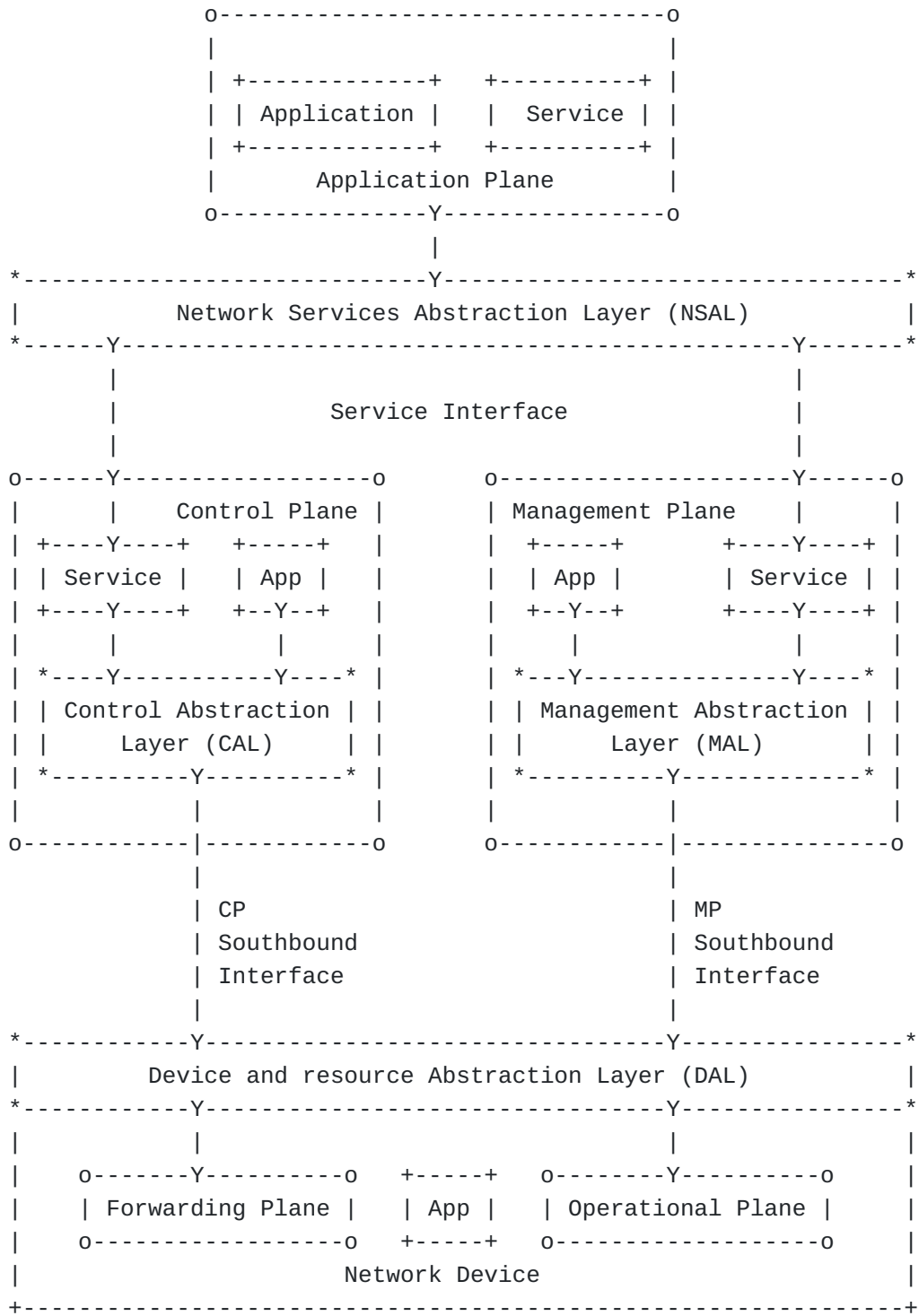
Figure 10: SDN Layers and Architecture Terminology per RFC 7426
