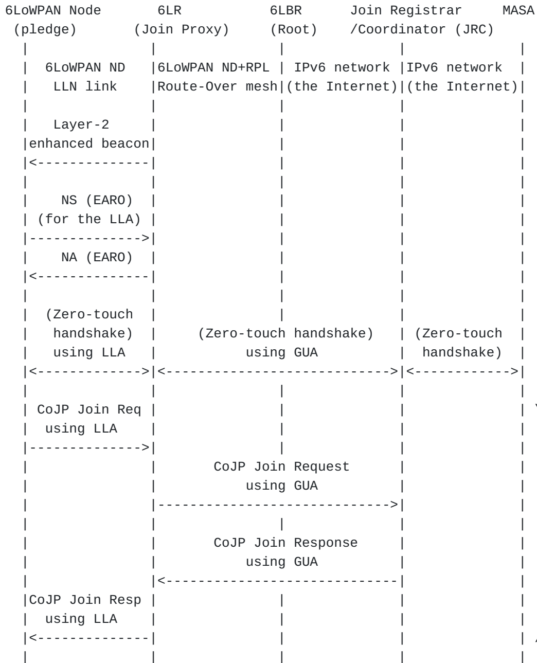
Figure 5: Join process in a Multi-Link Subnet. Parentheses ( ) denote optional exchanges.
