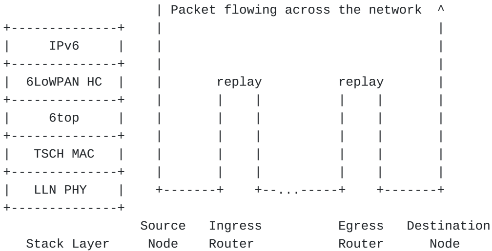
Figure 16: Forwarding Next Fragment
