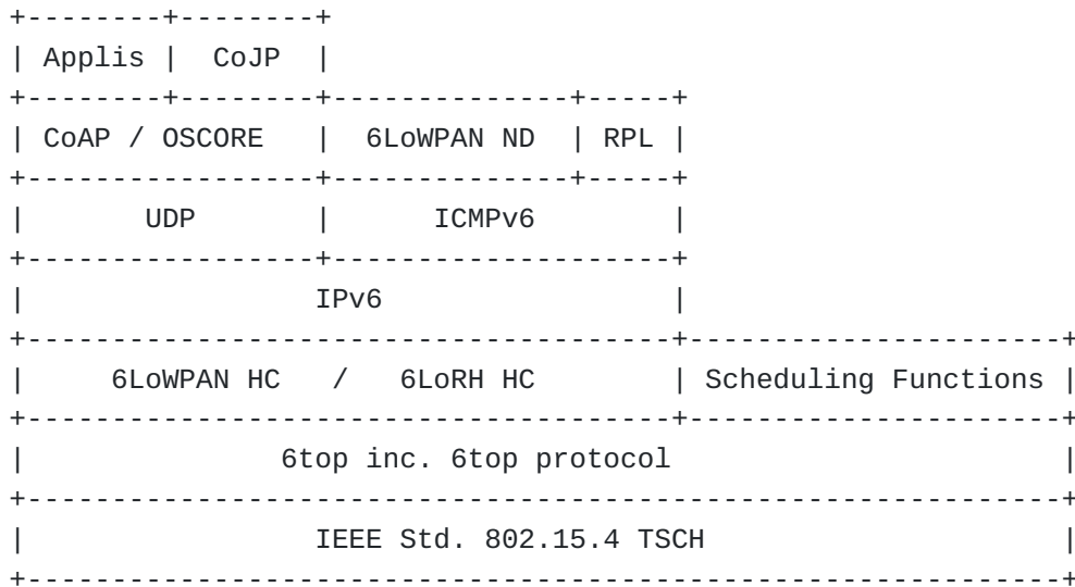
Figure 4: 6TiSCH Protocol Stack
