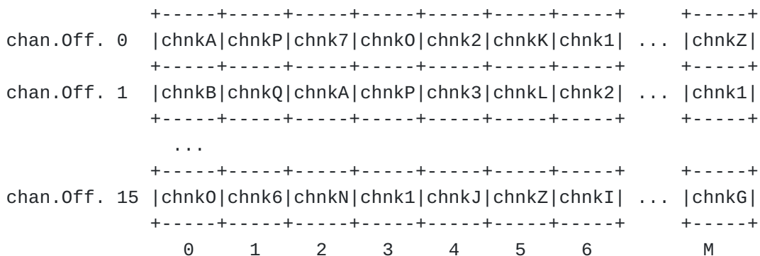
Figure 9: CDU matrix Partitioning in Chunks
