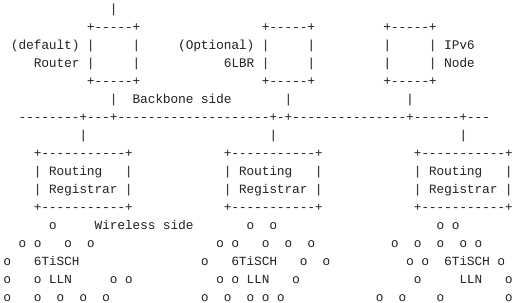
Figure 2: Extended Configuration of a 6TiSCH Network
