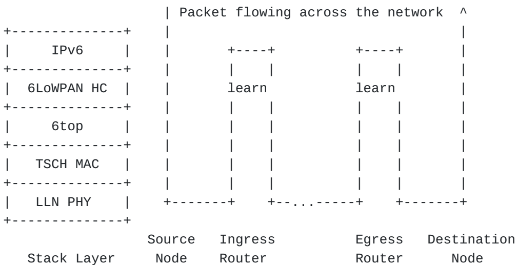
Figure 15: Forwarding First Fragment
