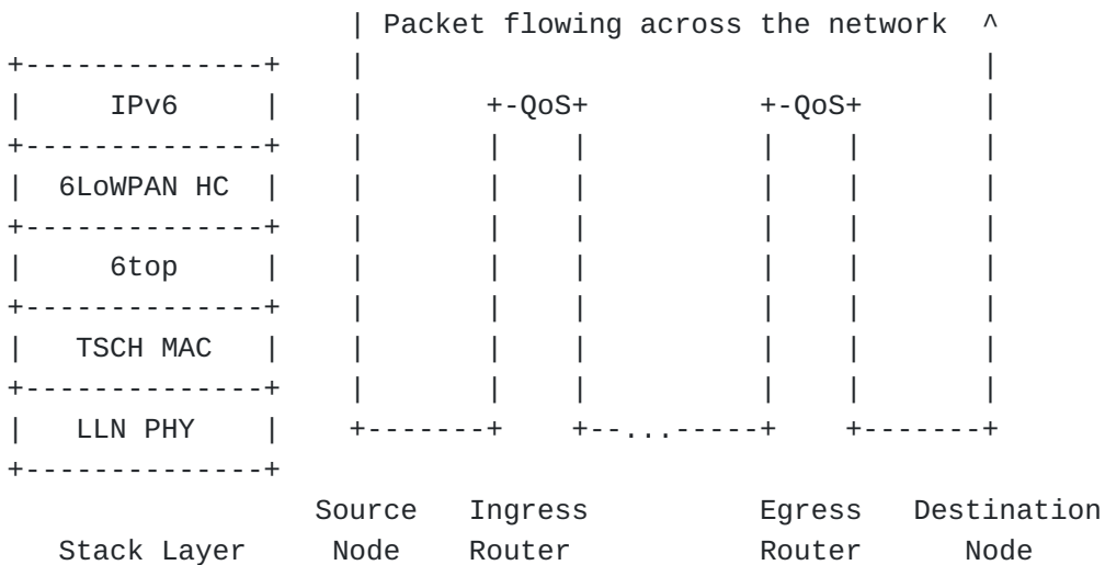
Figure 14: IP Forwarding
