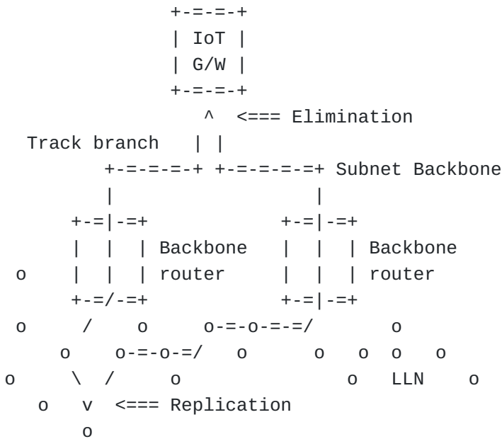
Figure 11: Example End-to-End DetNet Track
