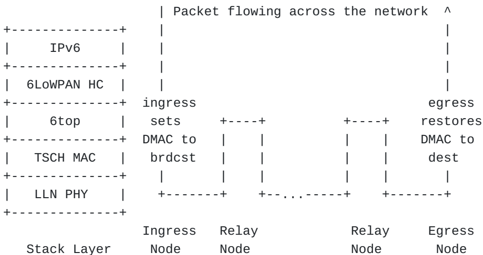
Figure 12: Track Forwarding, Native Mode
