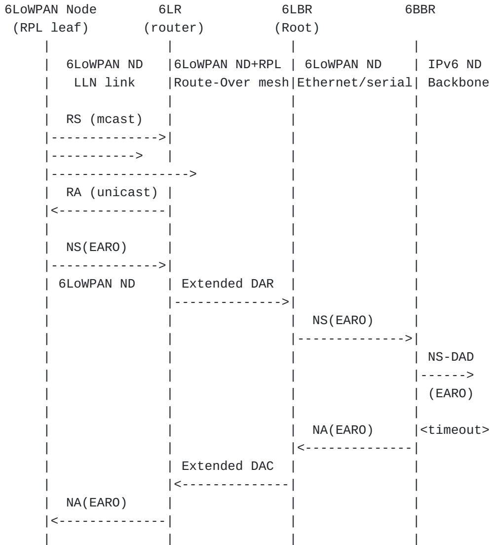
Figure 6: Initial Registration Flow over Multi-Link Subnet
