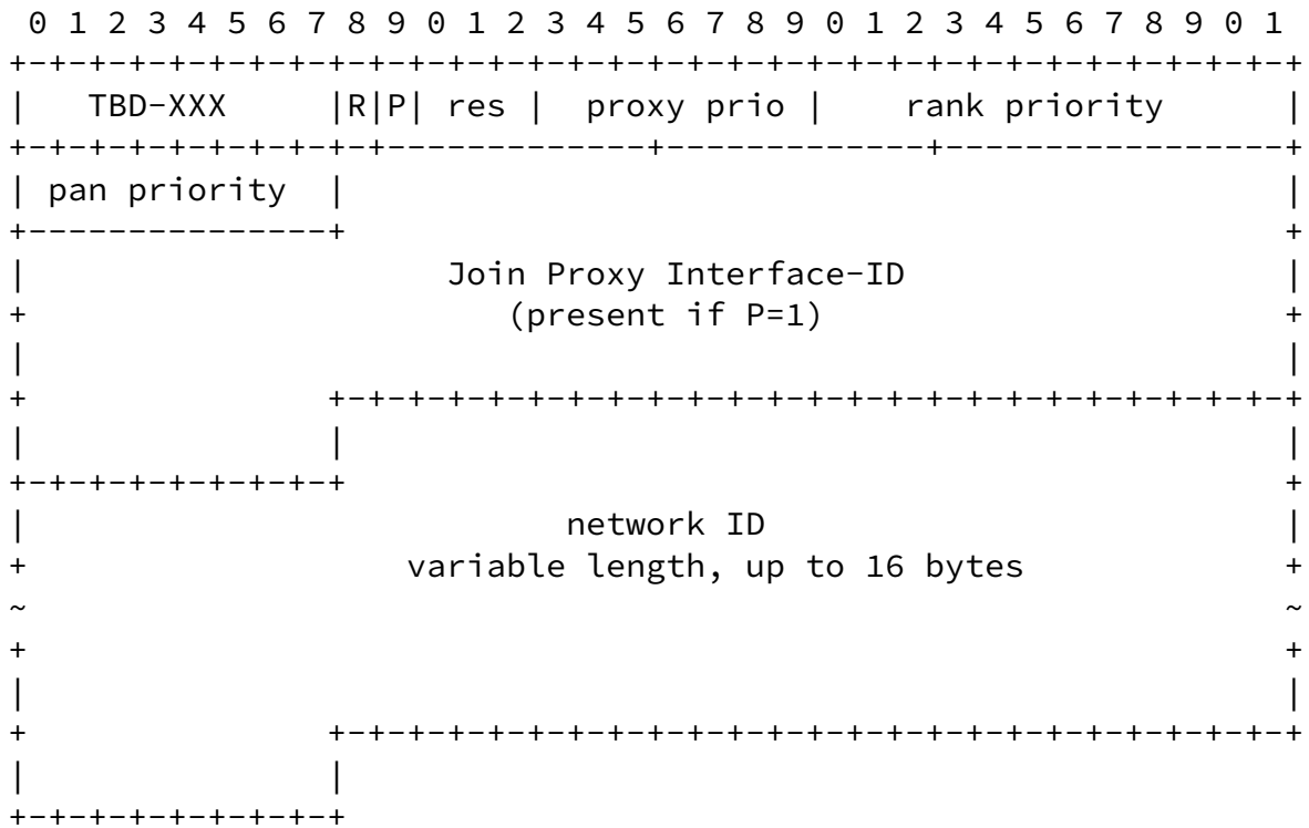
Figure 1: IE subtype structure
