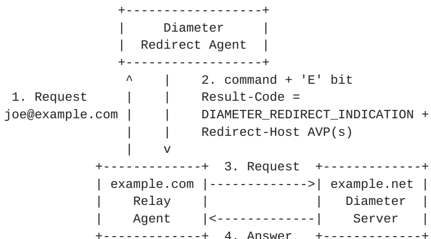
Figure 6: Diameter Redirect Agent
