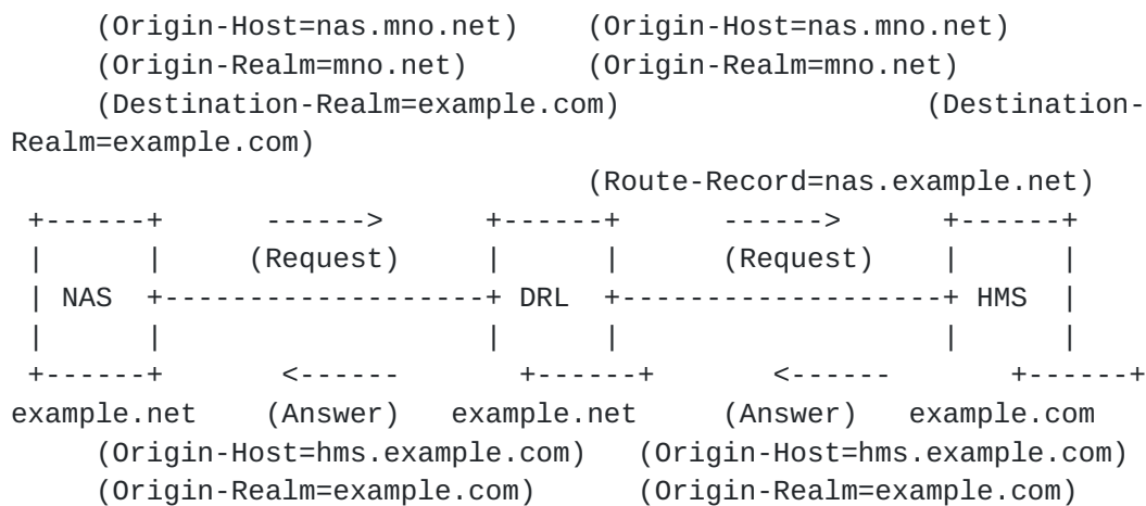
Figure 7: Routing of Diameter messages
