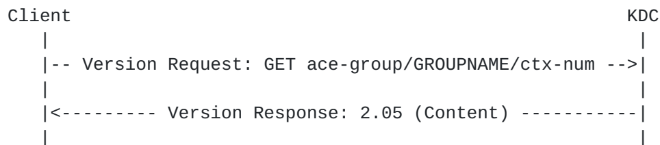
Figure 15: Message Flow of Version Request-Response
