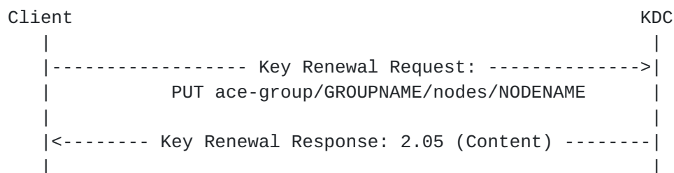
Figure 10: Message Flow of Key Renewal Request-Response
