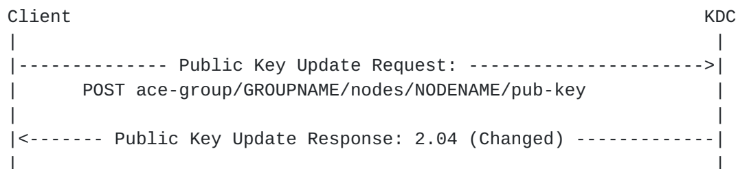
Figure 22: Message Flow of Public Key Update Request-Response
