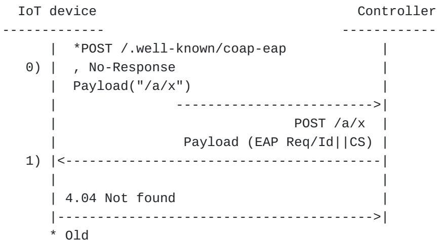
Figure 5: /.well-known/coap-eap with no ongoing authentication from the EAP authenticator
