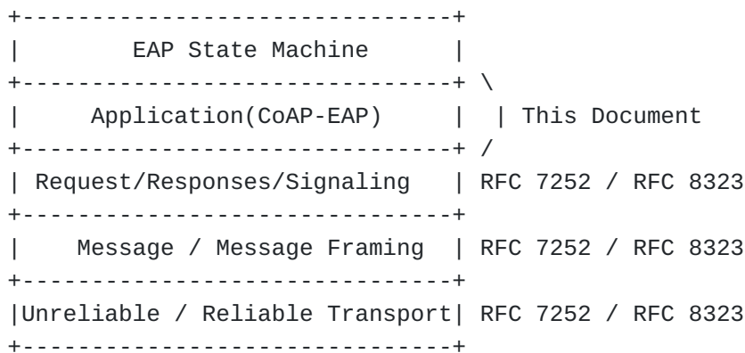
Figure 2: CoAP-EAP Stack
