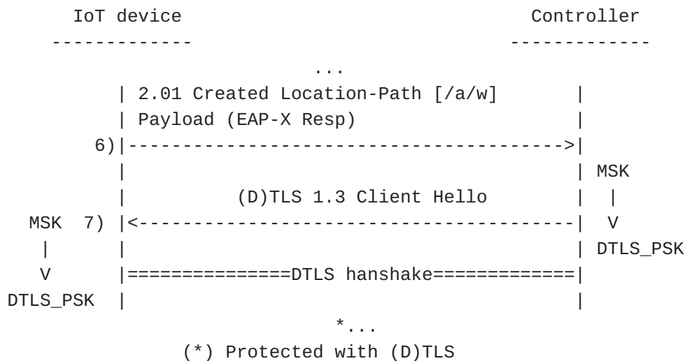
Figure 10: CoAP-EAP flow of operation with DTLS
