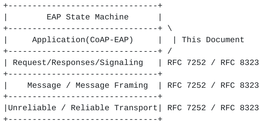
Figure 2: CoAP-EAP Stack
