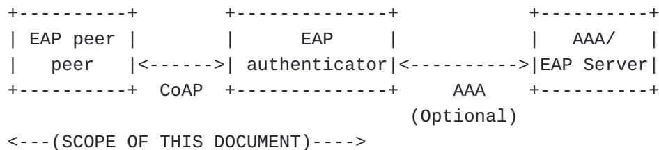
Figure 1: CoAP-EAP Architecture
