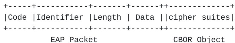
Figure 7: cipher suites are in the CoAP payload
