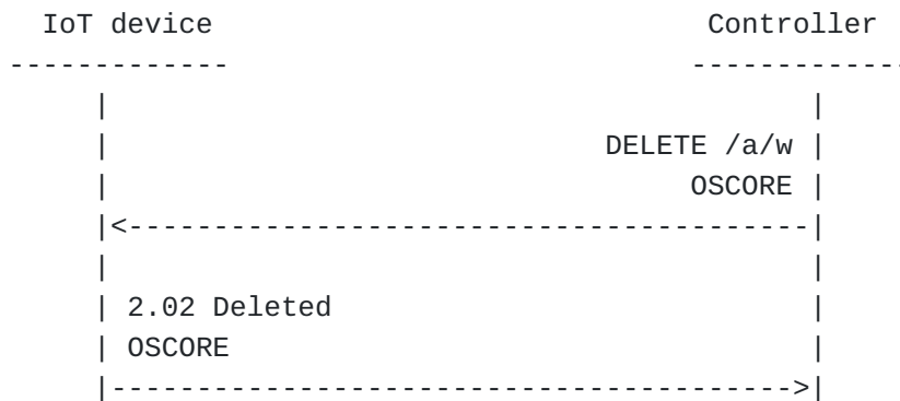
Figure 4: Deleting state
