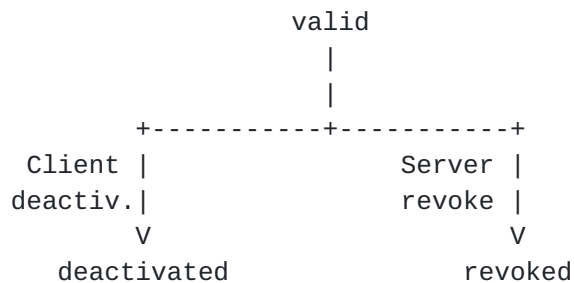
State Transitions for Account Objects
