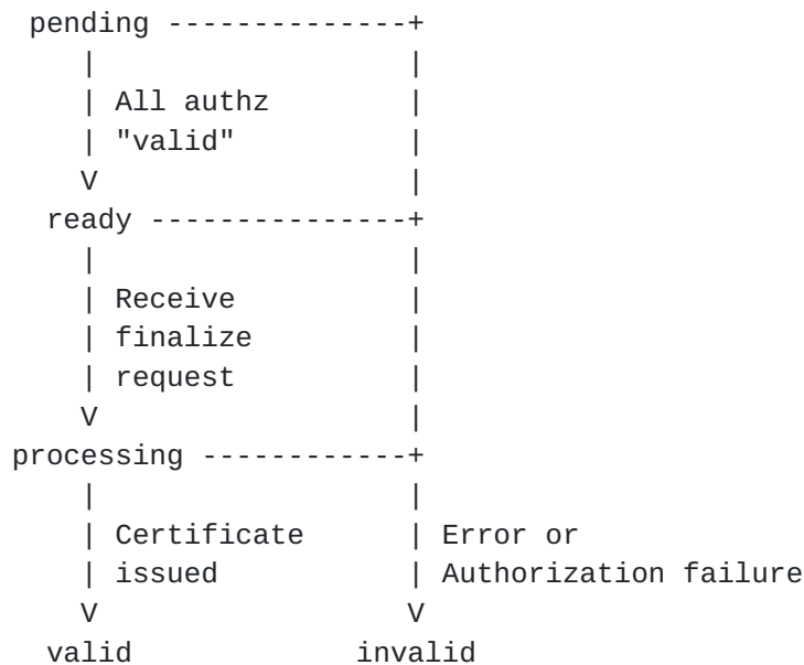
State Transitions for Order Objects
