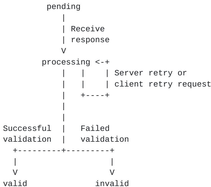
State Transitions for Challenge Objects
