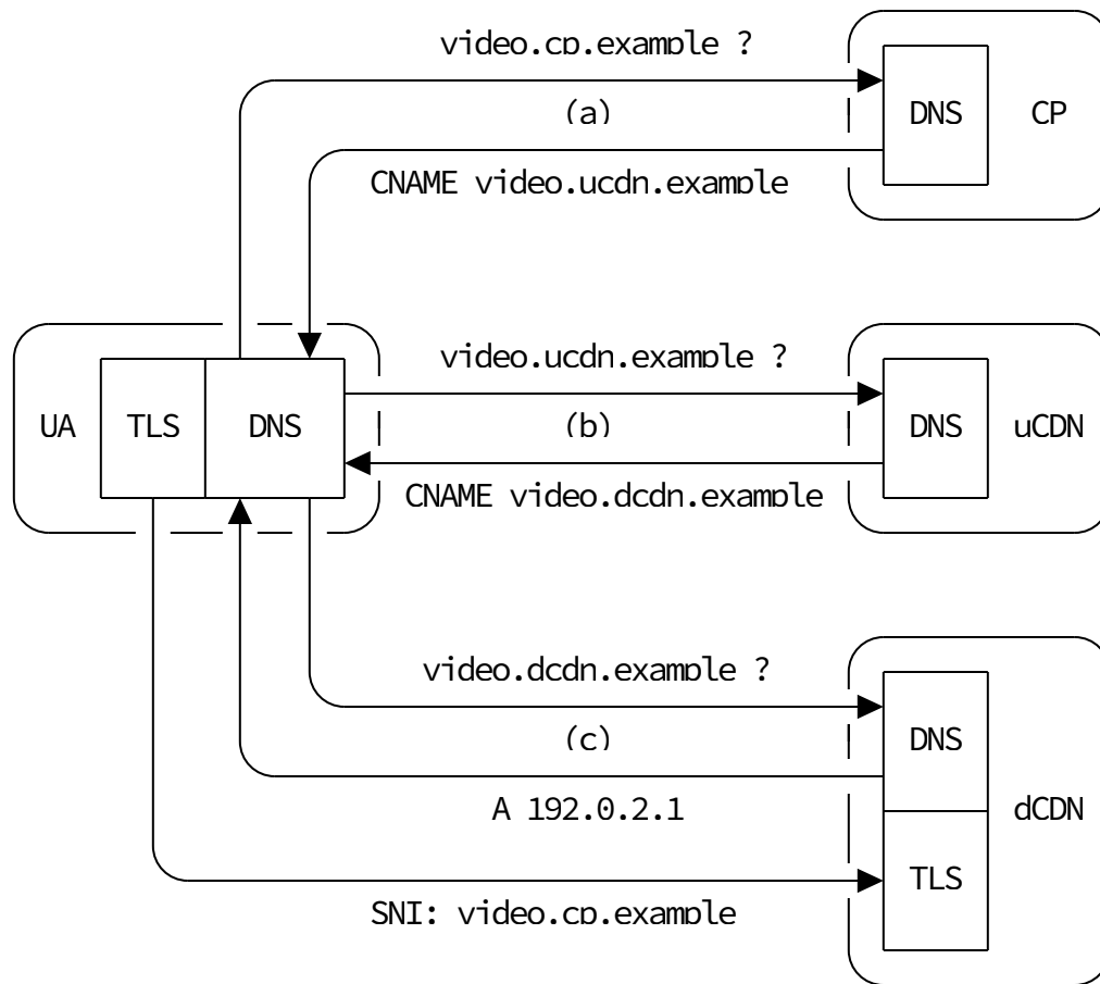
Figure 11: DNS Redirection
