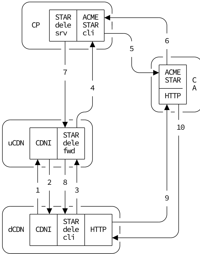
Figure 12: Two levels delegation in CDNI
