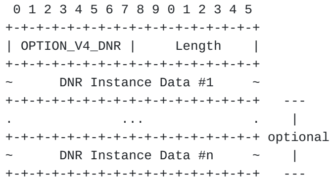
Figure 4: DHCPv4 Encrypted DNS Option
