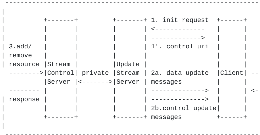
Figure 2: ALTO SSE Architecture and Message Flow.
