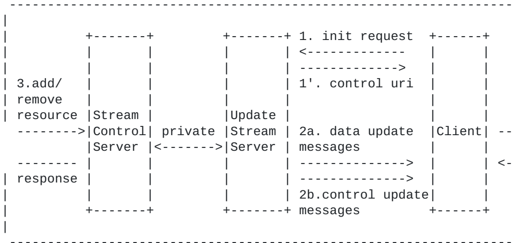
Figure 2: ALTO SSE Architecture and Message Flow.
