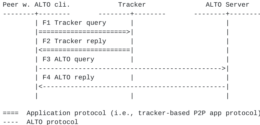
Figure 2: Basic message sequence chart for resource consumer-initiated ALTO query
