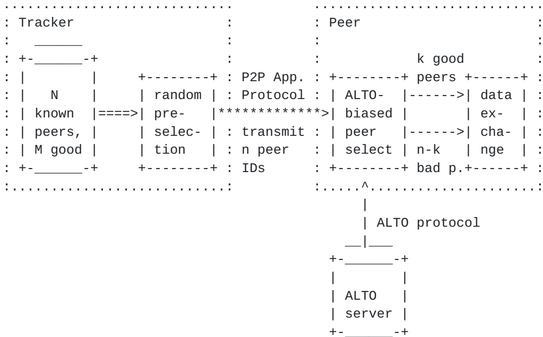
Figure 1: Tracker-based P2P Application with random peer preselection
