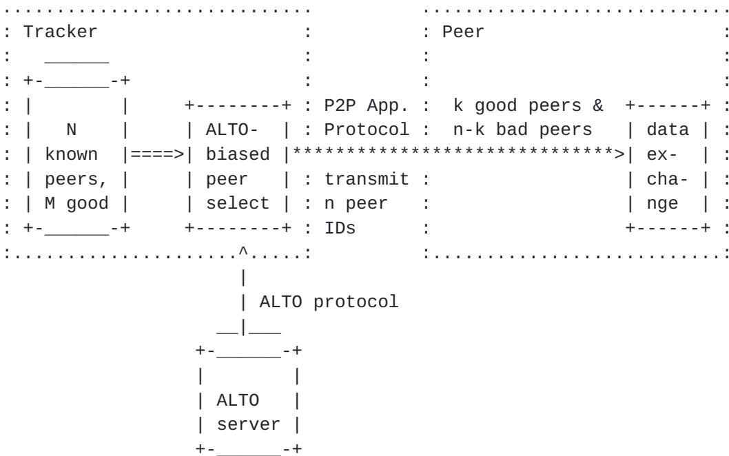
Figure 3: Tracker-based P2P Application with ALTO client in tracker
