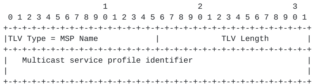
Figure 7: Multicast-Service-Profile-Name TLV
