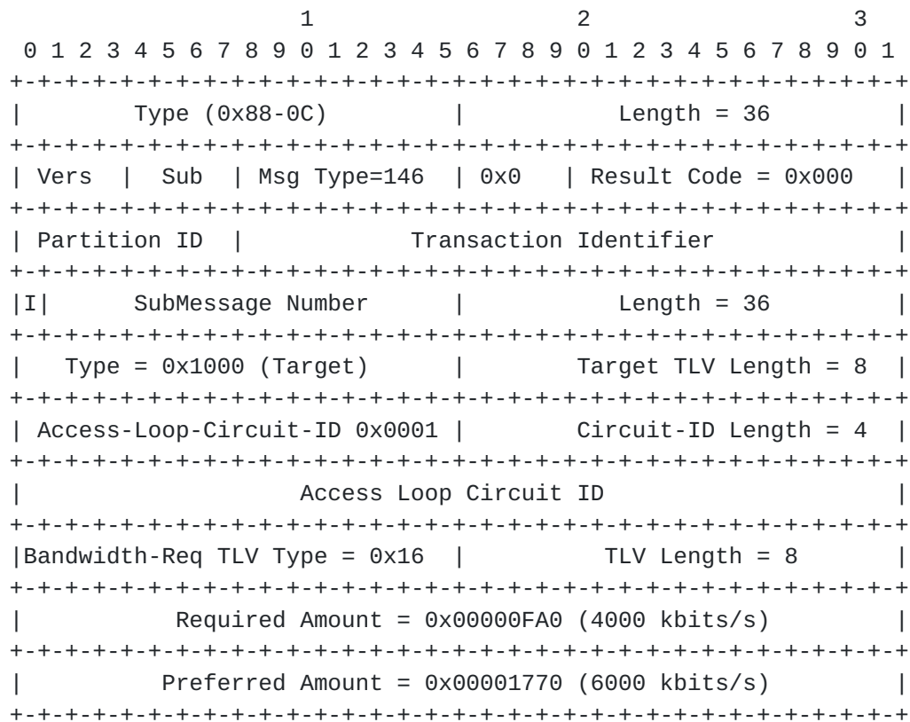
Figure 26: Bandwidth Reallocation Request Message
