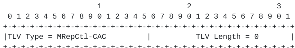
Figure 13: MRepCtl-CAC TLV
