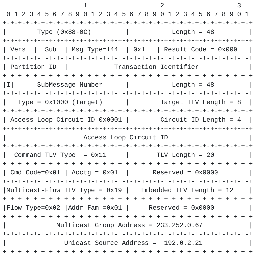
Figure 24: Multicast Replication Control Message Admitting A Flow
