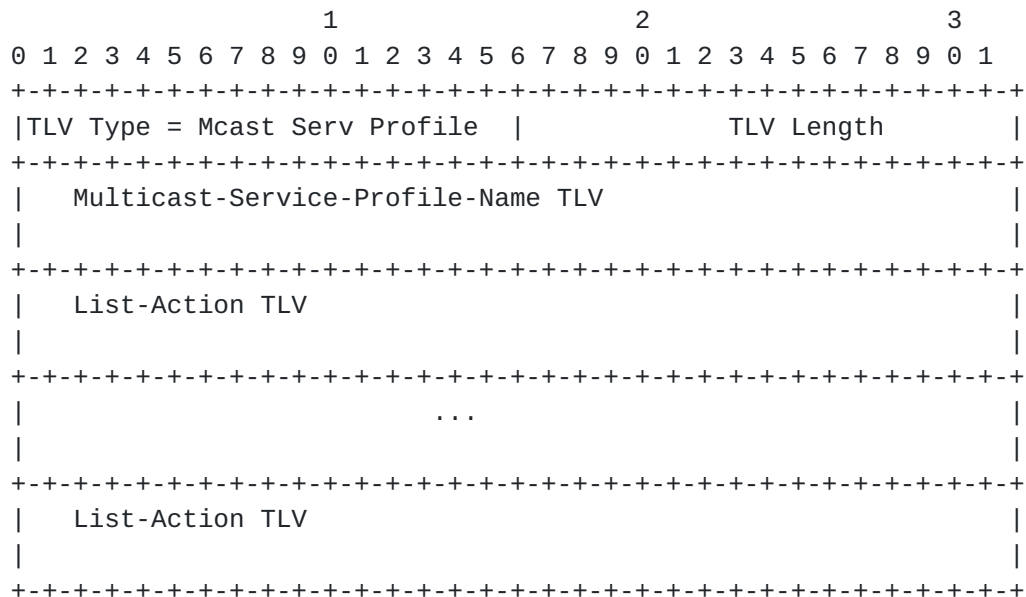
Figure 6: Multicast-Service-Profile TLV
