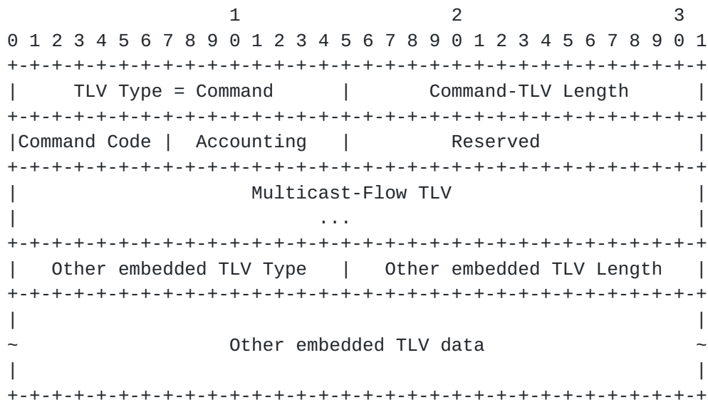
Figure 5: Contents of the Command TLV in the Multicast Replication Control Message
