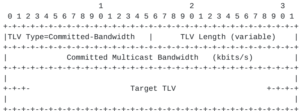
Figure 19: Committed-Bandwidth TLV
