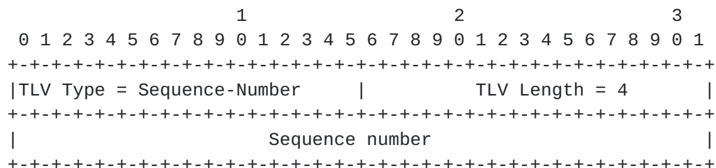
Figure 10: Sequence-Number TLV
