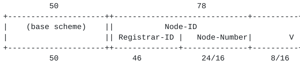
Figure 11: ACP Vlong Addressing Sub-Scheme
