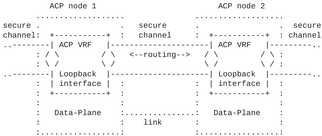
Figure 1: ACP VRF and secure channels
