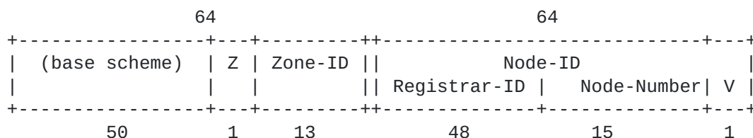
Figure 9: ACP Zone Addressing Sub-Scheme
