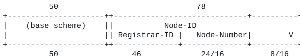
Figure 11: ACP Vlong Addressing Sub-Scheme
