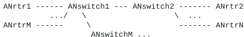
Figure 13: Topology with L2 ACP switches
