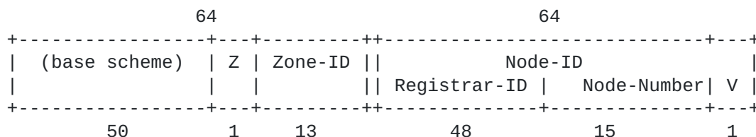
Figure 10: ACP Zone Addressing Sub-Scheme
