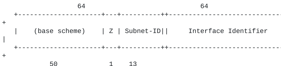
Figure 11: ACP Manual Addressing Sub-Scheme
