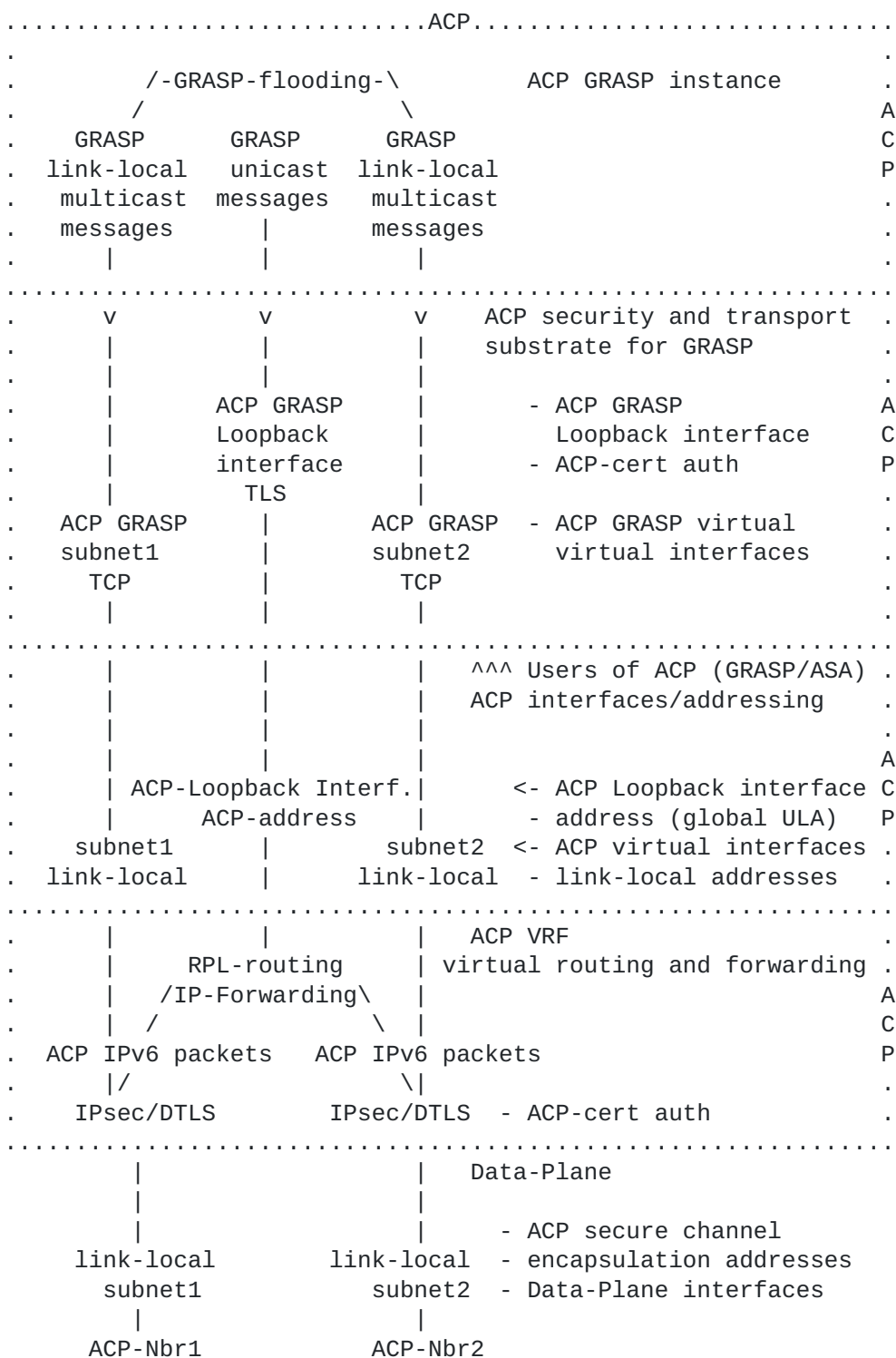
Figure 8: ACP as security and transport substrate for GRASP
