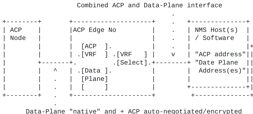
Figure 15: VRF select
