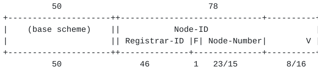
Figure 14: ACP Vlong Addressing Sub-Scheme
