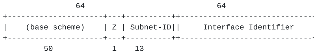
Figure 13: ACP Manual Addressing Sub-Scheme
