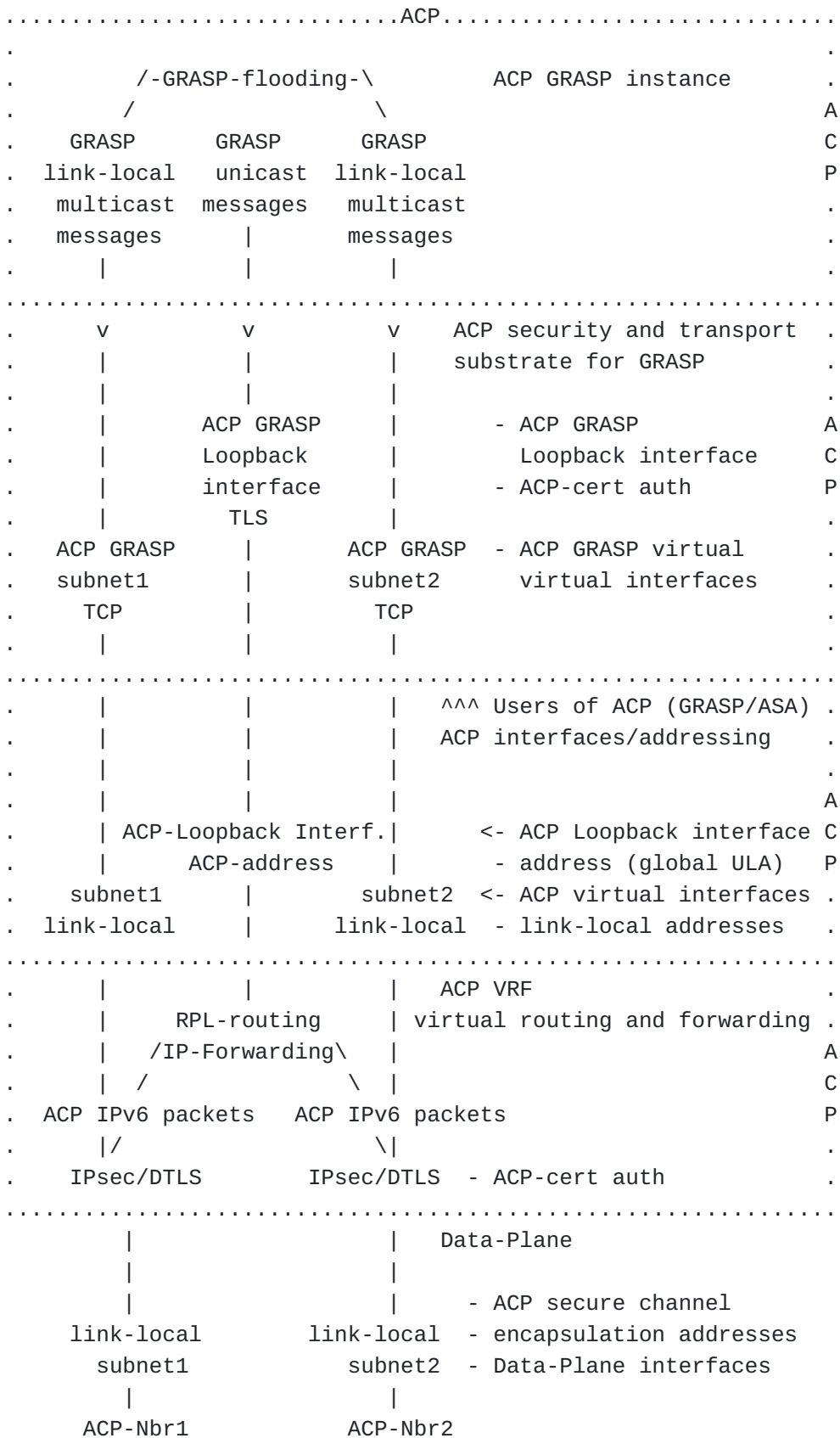
Figure 9: ACP as security and transport substrate for GRASP
