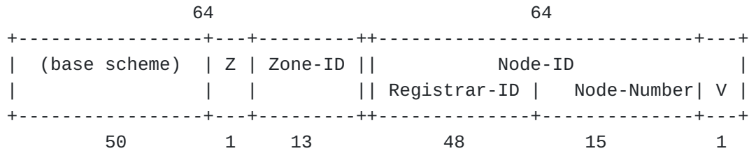
Figure 12: ACP Zone Addressing Sub-Scheme
