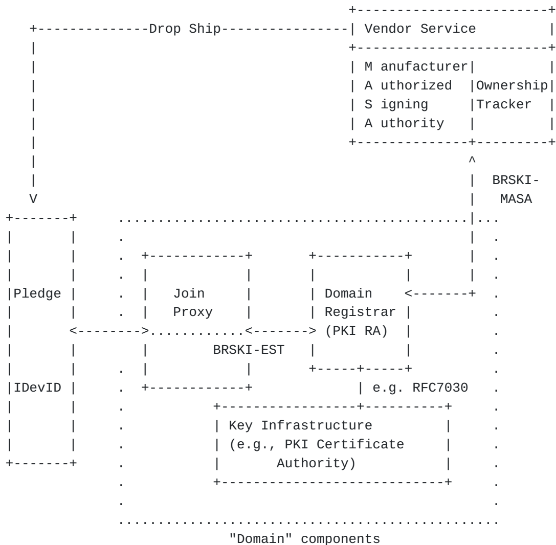
Figure 1: Architecture Overview
