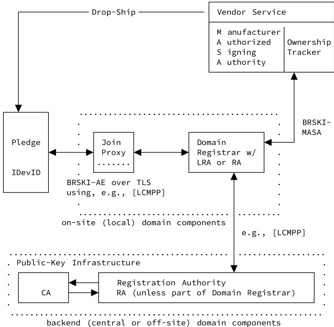
Figure 1: Architecture Overview Using Backend PKI Components
