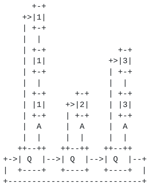
Figure 1: Round Robin Queues
