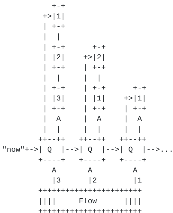
Figure 2: Calendar Queue
