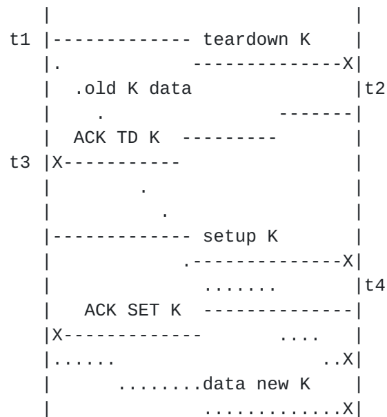
Figure 4: Channel ID Reuse Problem
