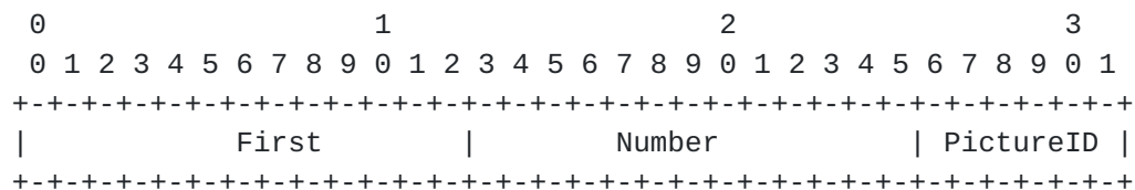
Figure 6: Syntax of the Slice Lost Indication (SLI)
