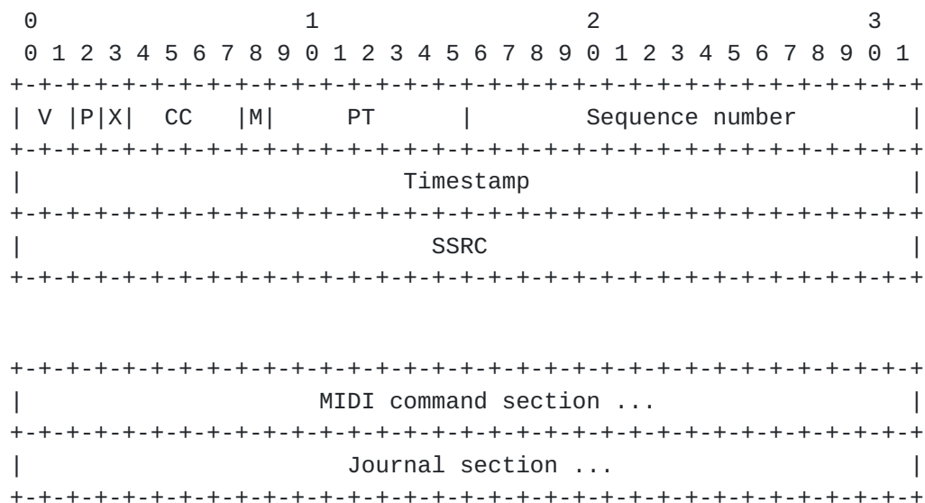
Figure 1 -- Packet format
