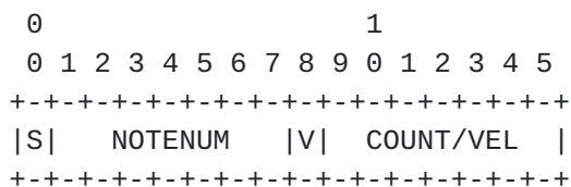
Figure A.7.2 -- Chapter E note log
