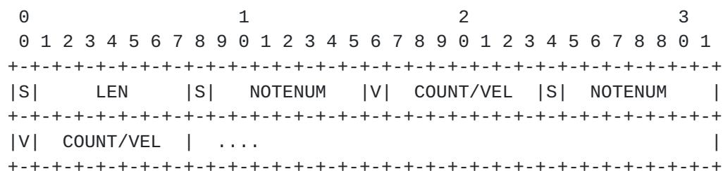
Figure A.7.1 -- Chapter E format
