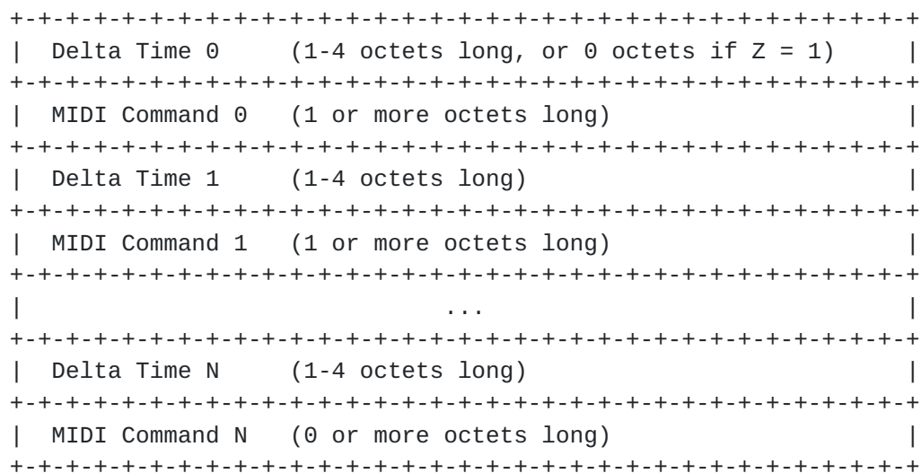
Figure 3 -- MIDI list structure.
