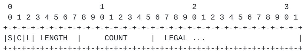
Figure B.1.5 -- Undefined System Real-time command log format
