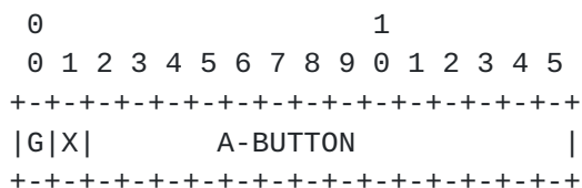
Figure A.4.5 -- A-BUTTON field
