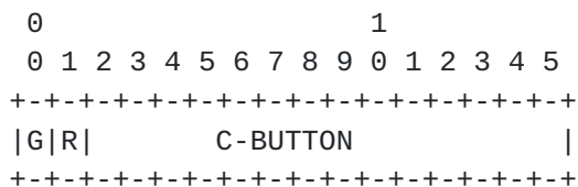
Figure A.4.6 -- C-BUTTON field
