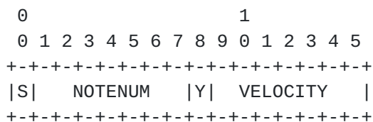
Figure A.6.3 -- Chapter N note log
