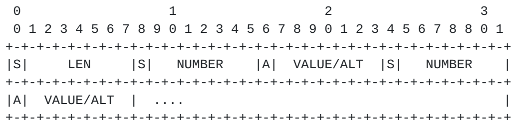
Figure A.3.1 -- Chapter C format
