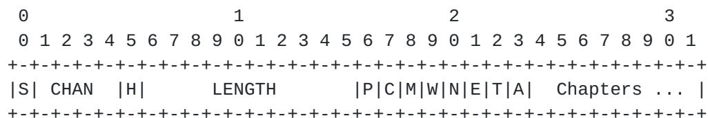
Figure 9 -- Channel journal format
