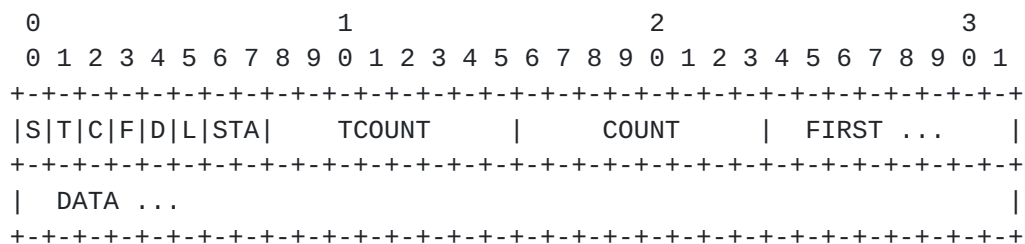
Figure B.5.1 -- Chapter X command log format
