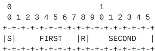
Figure A.5.1 -- Chapter W format
