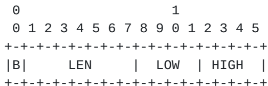
Figure A.6.2 -- Chapter N header
