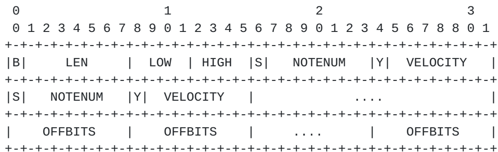
Figure A.6.1 -- Chapter N format
