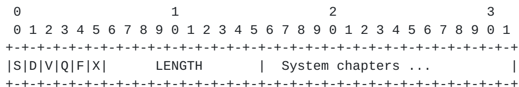
Figure 10 -- System journal format
