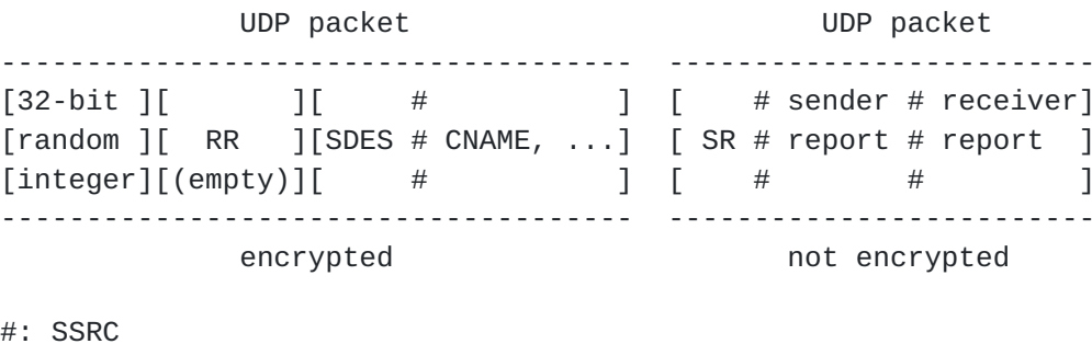
Figure 4: Encrypted and non-encrypted RTCP packets
