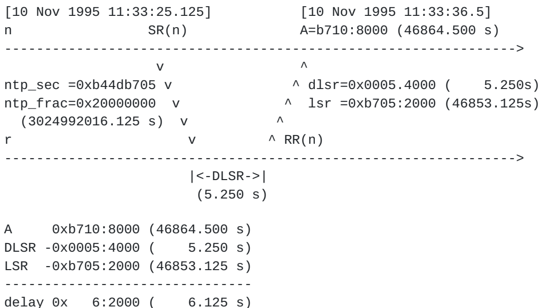
Figure 2: Example for round-trip time computation
