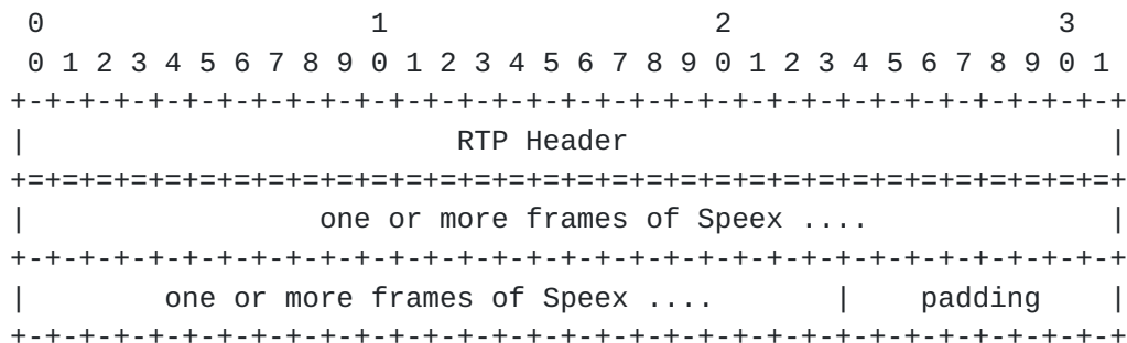
Figure 1: RTP payload for Speex
