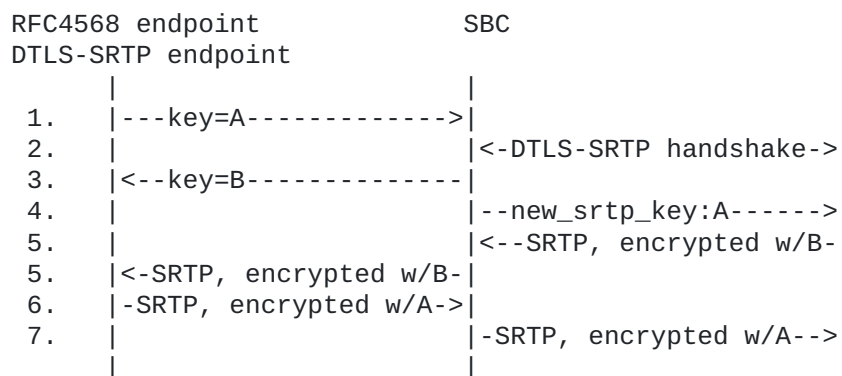
Figure 12: Interworking Security Descriptions and EKT
