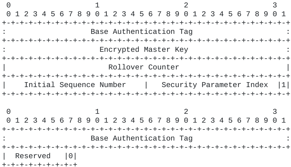
Figure 1: The EKT Authentication Tag format.
