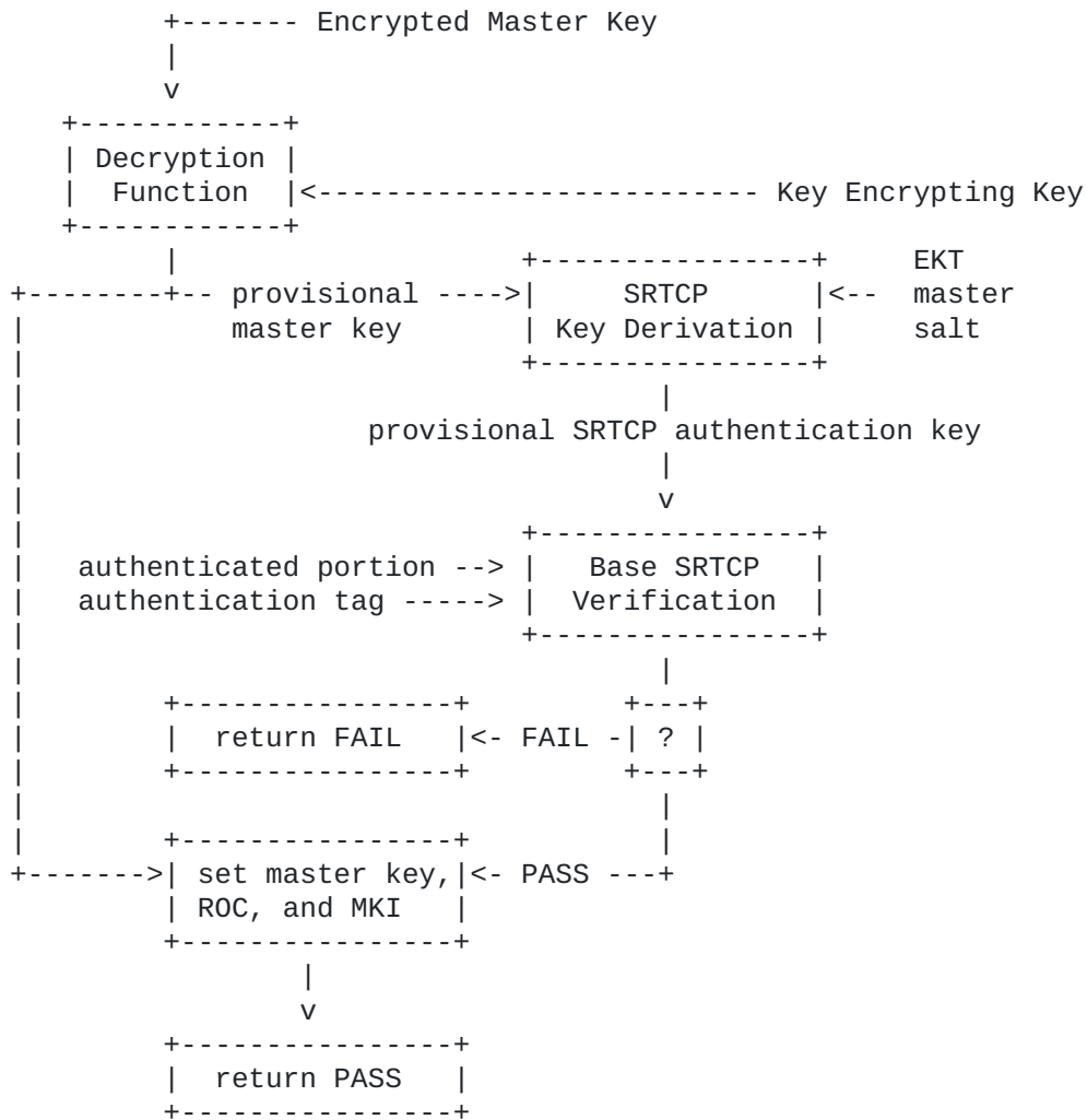
Figure 2: EKT inbound processing.
