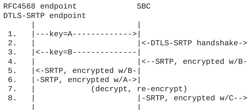
Figure 11: Interworking Security Descriptions and DTLS-SRTP
