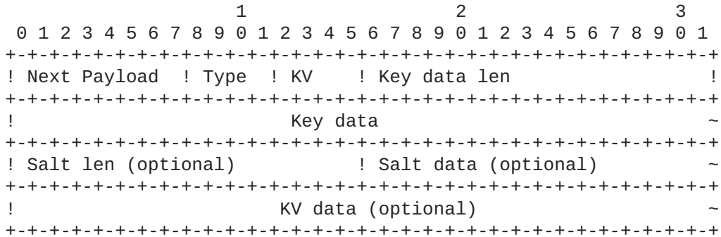
Figure 10: Key Data Sub-Payload of MIKEY
