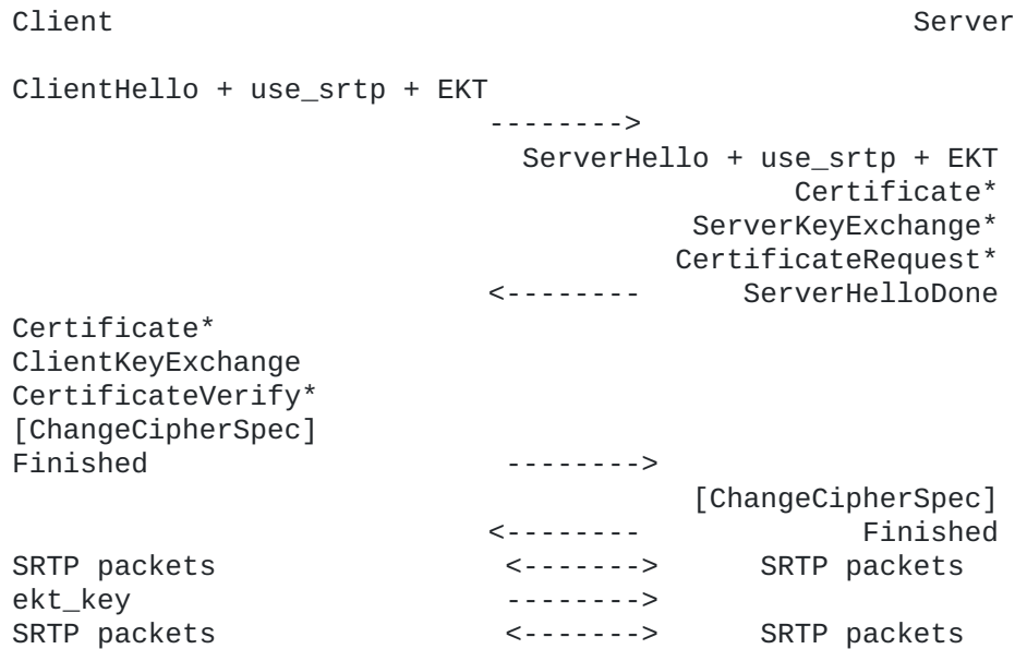
Figure 6: Handshake Message Flow
